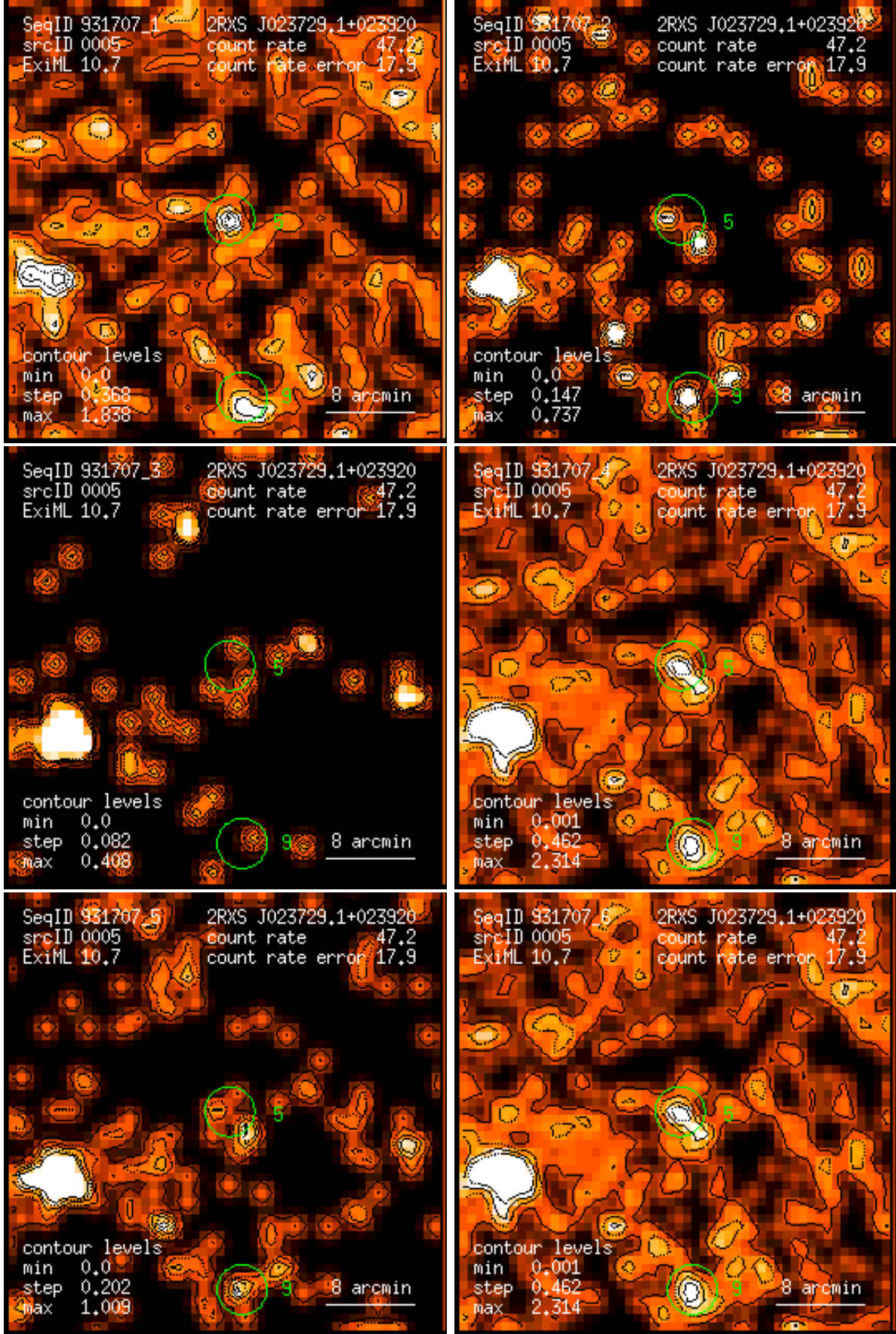
Figure 5: RASS 931707: detection 0005: band rate images, Gaussian filter: (1) PSPC channels 11 – 41, (2) 52 – 90, (3) 91 – 201, (4) 11 – 235, (5) 52 – 201, (6) 11 – 201. Broad band rates in counts/ks. Band rate contour levels in counts/ks/arcmin 2 .
