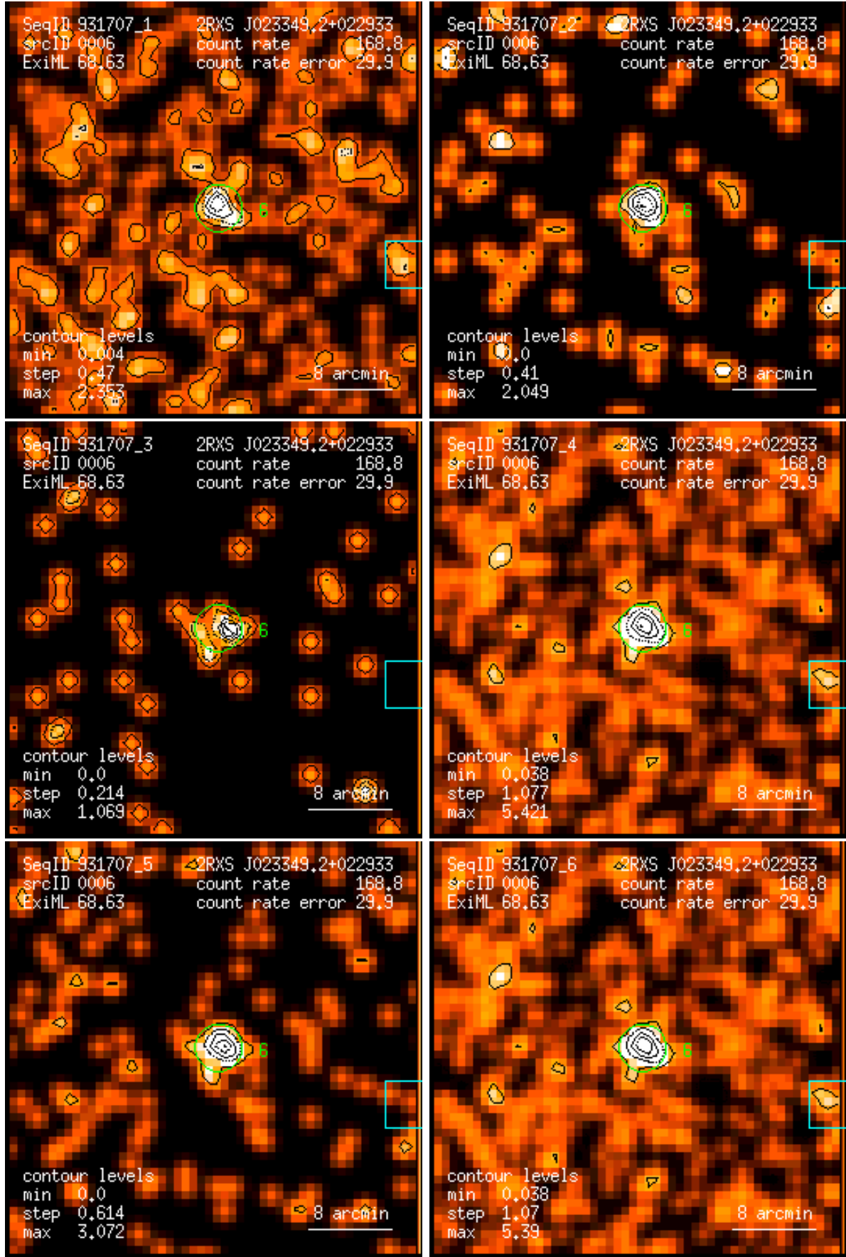
Figure 6: RASS 931707: detection 0006: band rate images, Gaussian filter: (1) PSPC channels 11 – 41, (2) 52 – 90, (3) 91 – 201, (4) 11 – 235, (5) 52 – 201, (6) 11 – 201. Broad band rates in counts/ks. Band rate contour levels in counts/ks/arcmin 2 .
