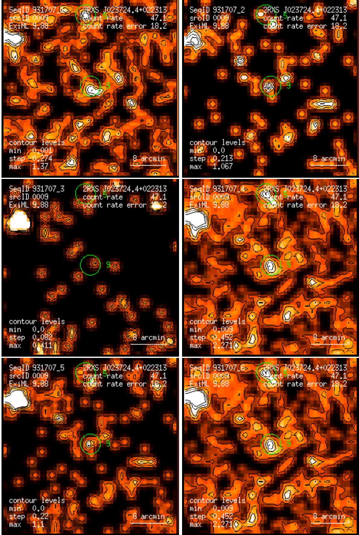
Figure 9: RASS 931707: detection 0009: band rate images, Gaussian filter: (1) PSPC channels 11 – 41, (2) 52 – 90, (3) 91 – 201, (4) 11 – 235, (5) 52 – 201, (6) 11 – 201. Broad band rates in counts/ks. Band rate contour levels in counts/ks/arcmin 2 .
