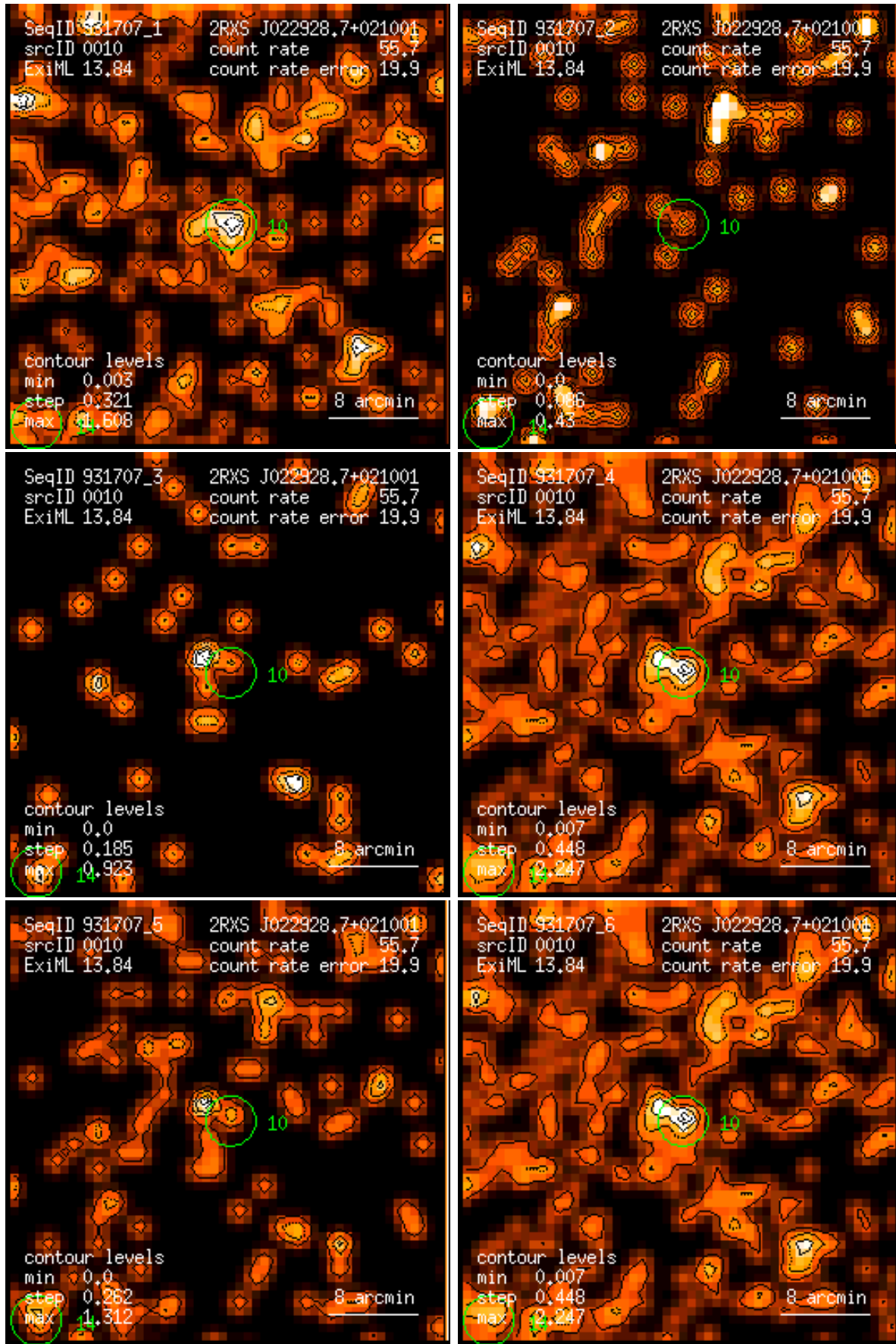
Figure 10: RASS 931707: detection 0010: band rate images, Gaussian filter: (1) PSPC channels 11 – 41, (2) 52 – 90, (3) 91 – 201, (4) 11 – 235, (5) 52 – 201, (6) 11 – 201. Broad band rates in counts/ks. Band rate contour levels in counts/ks/arcmin 2 .
