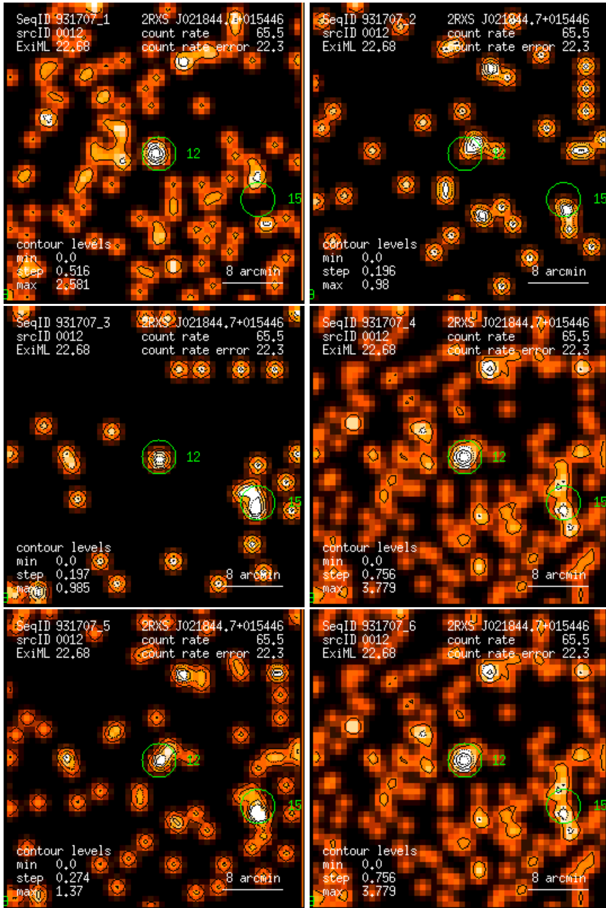
Figure 12: RASS 931707: detection 0012: band rate images, Gaussian filter: (1) PSPC channels 11 – 41, (2) 52 – 90, (3) 91 – 201, (4) 11 – 235, (5) 52 – 201, (6) 11 – 201. Broad band rates in counts/ks. Band rate contour levels in counts/ks/arcmin 2 .
