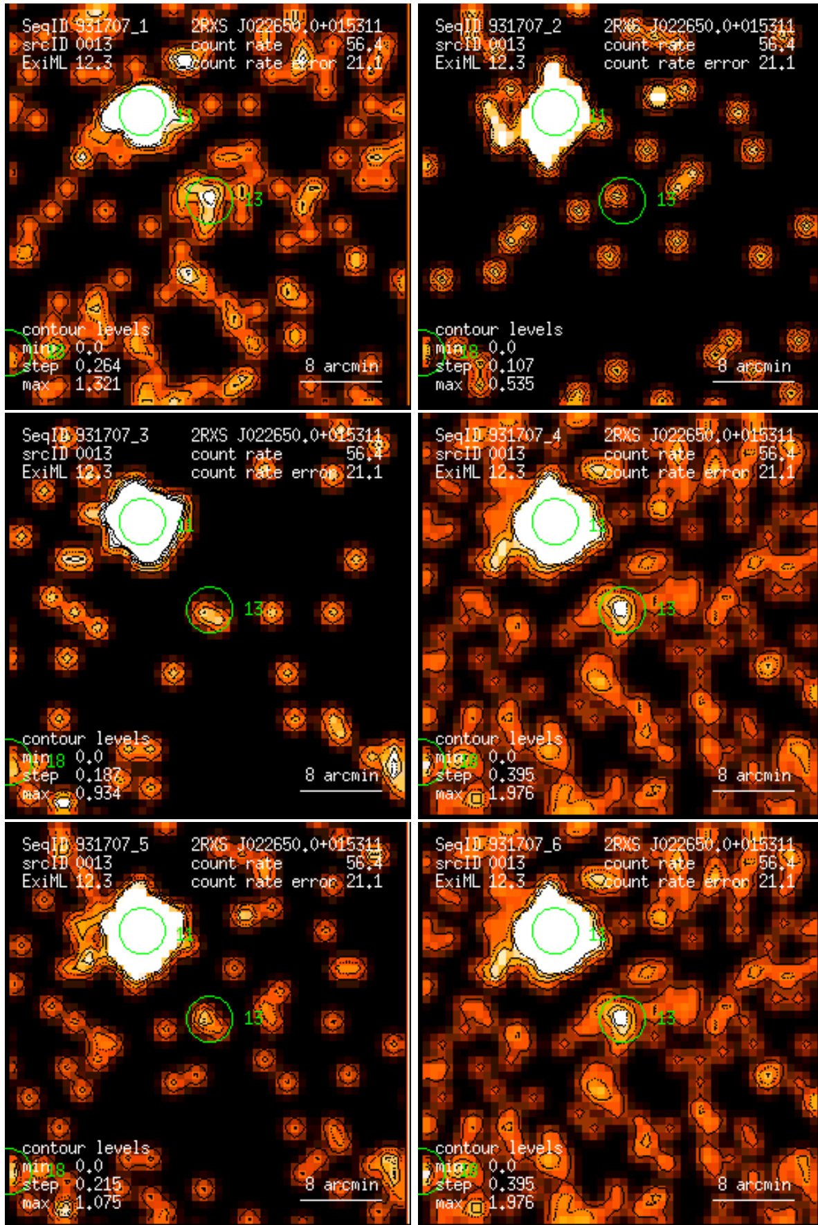
Figure 13: RASS 931707: detection 0013: band rate images, Gaussian filter: (1) PSPC channels 11 – 41, (2) 52 – 90, (3) 91 – 201, (4) 11 – 235, (5) 52 – 201, (6) 11 – 201. Broad band rates in counts/ks. Band rate contour levels in counts/ks/arcmin 2 .
