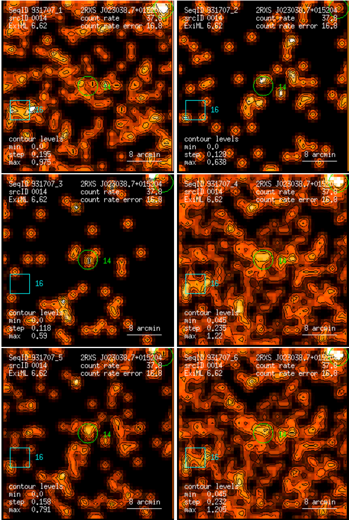
Figure 14: RASS 931707: detection 0014: band rate images, Gaussian filter: (1) PSPC channels 11 – 41, (2) 52 – 90, (3) 91 – 201, (4) 11 – 235, (5) 52 – 201, (6) 11 – 201. Broad band rates in counts/ks. Band rate contour levels in counts/ks/arcmin 2 .
