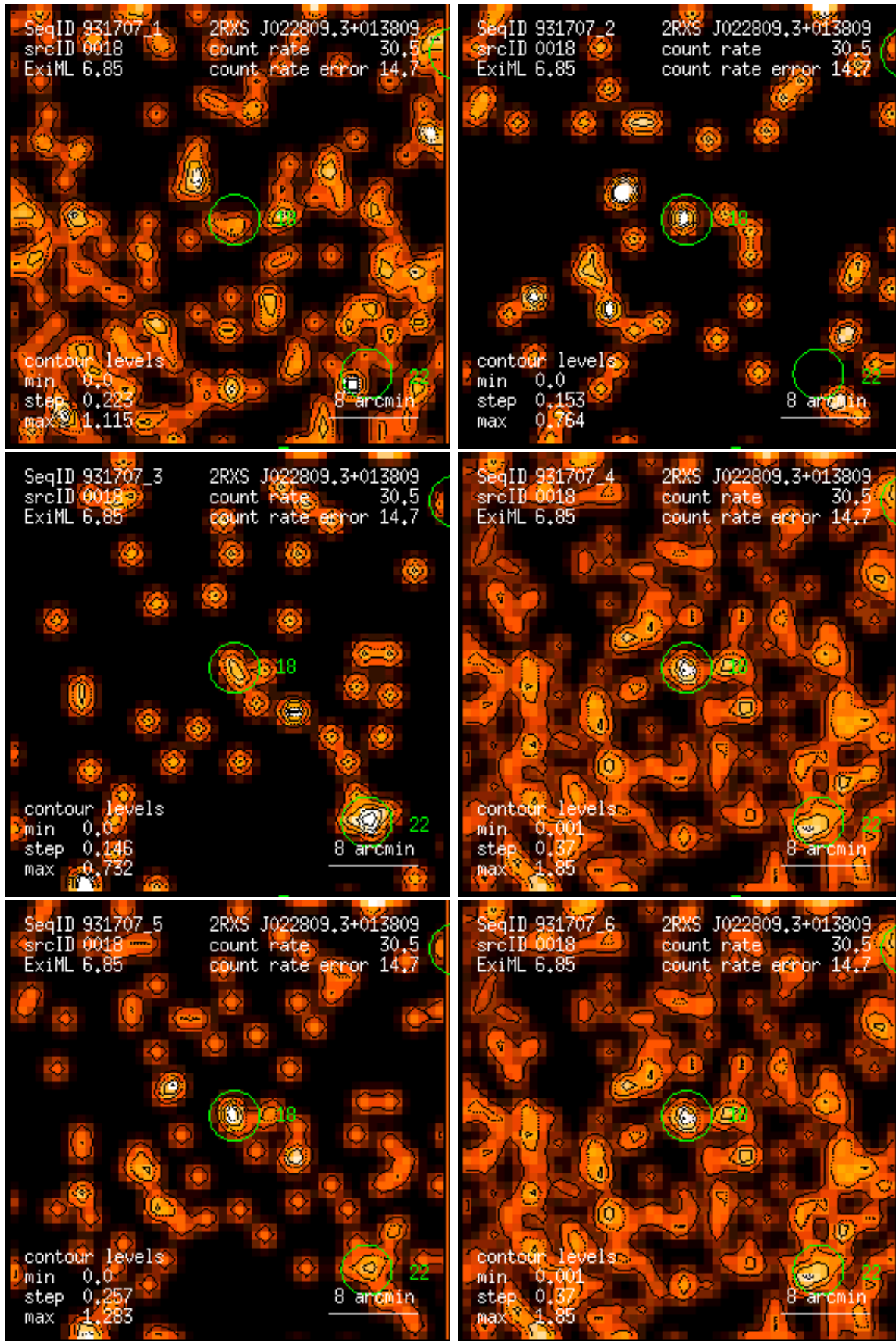
Figure 18: RASS 931707: detection 0018: band rate images, Gaussian filter: (1) PSPC channels 11 – 41, (2) 52 – 90, (3) 91 – 201, (4) 11 – 235, (5) 52 – 201, (6) 11 – 201. Broad band rates in counts/ks. Band rate contour levels in counts/ks/arcmin 2 .
