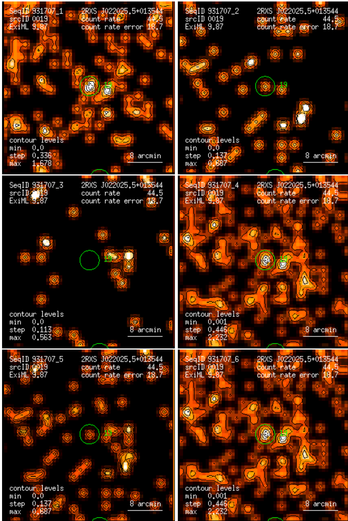
Figure 19: RASS 931707: detection 0019: band rate images, Gaussian filter: (1) PSPC channels 11 – 41, (2) 52 – 90, (3) 91 – 201, (4) 11 – 235, (5) 52 – 201, (6) 11 – 201. Broad band rates in counts/ks. Band rate contour levels in counts/ks/arcmin 2 .
