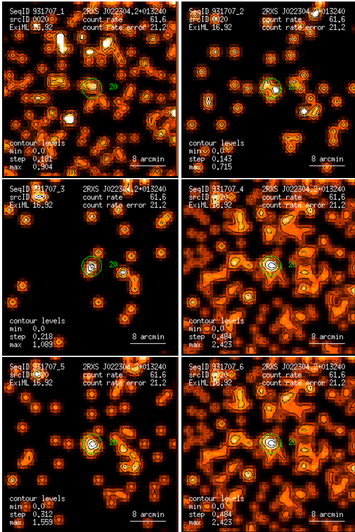
Figure 20: RASS 931707: detection 0020: band rate images, Gaussian filter: (1) PSPC channels 11 – 41, (2) 52 – 90, (3) 91 – 201, (4) 11 – 235, (5) 52 – 201, (6) 11 – 201. Broad band rates in counts/ks. Band rate contour levels in counts/ks/arcmin 2 .
