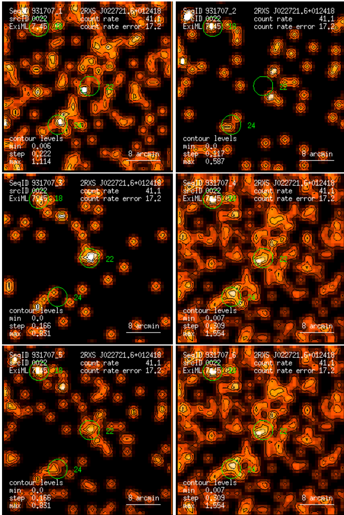
Figure 22: RASS 931707: detection 0022: band rate images, Gaussian filter: (1) PSPC channels 11 – 41, (2) 52 – 90, (3) 91 – 201, (4) 11 – 235, (5) 52 – 201, (6) 11 – 201. Broad band rates in counts/ks. Band rate contour levels in counts/ks/arcmin 2 .
