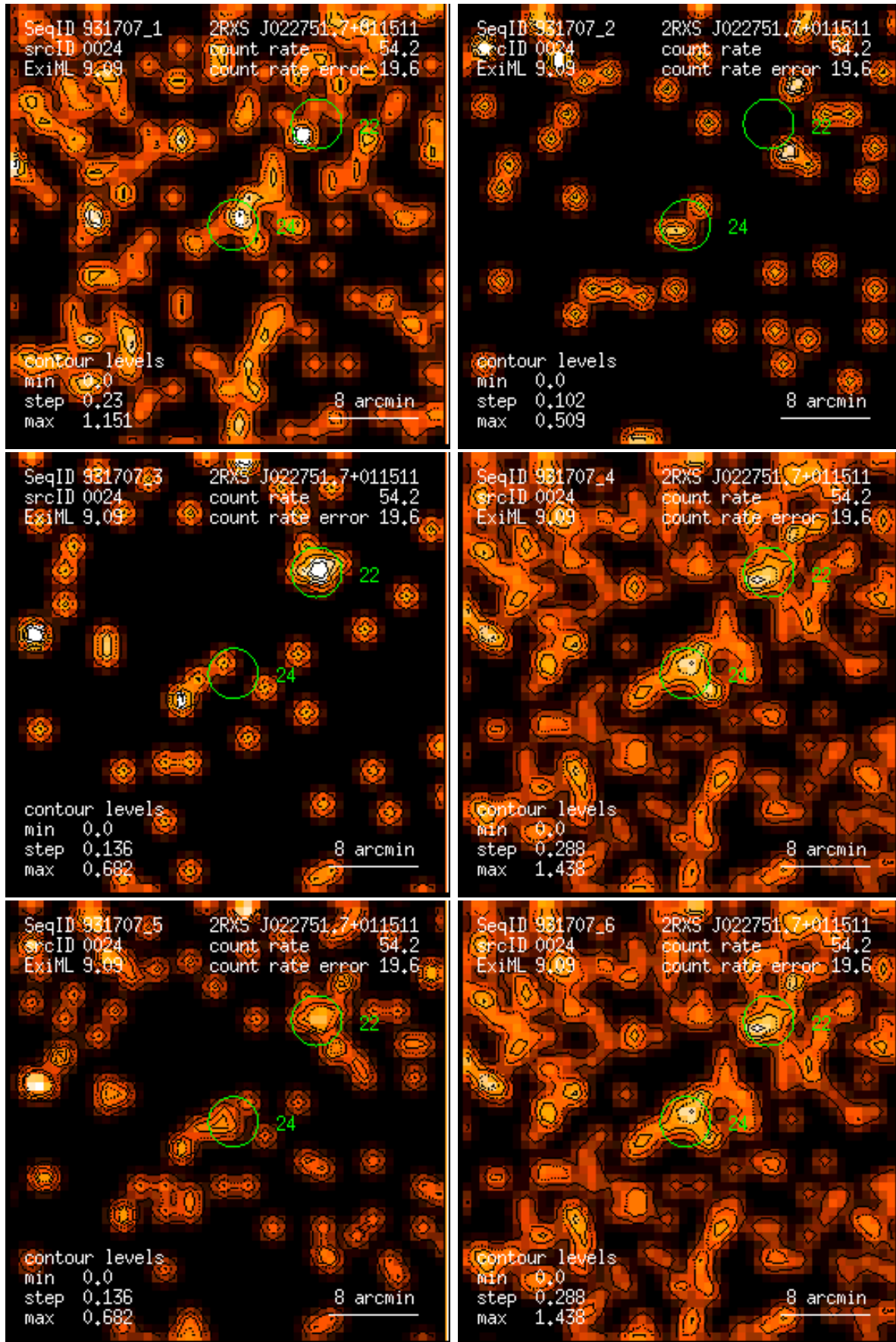
Figure 24: RASS 931707: detection 0024: band rate images, Gaussian filter: (1) PSPC channels 11 – 41, (2) 52 – 90, (3) 91 – 201, (4) 11 – 235, (5) 52 – 201, (6) 11 – 201. Broad band rates in counts/ks. Band rate contour levels in counts/ks/arcmin 2 .
