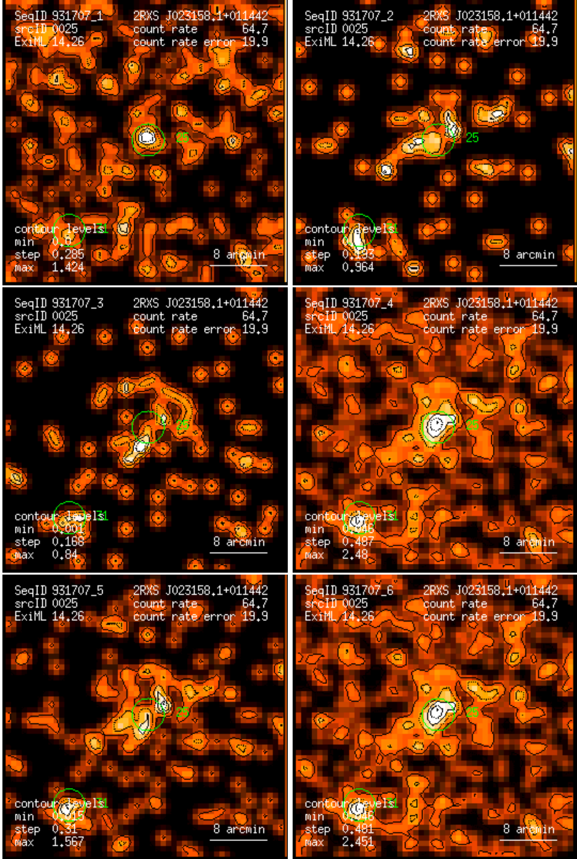
Figure 25: RASS 931707: detection 0025: band rate images, Gaussian filter: (1) PSPC channels 11 – 41, (2) 52 – 90, (3) 91 – 201, (4) 11 – 235, (5) 52 – 201, (6) 11 – 201. Broad band rates in counts/ks. Band rate contour levels in counts/ks/arcmin 2 .
