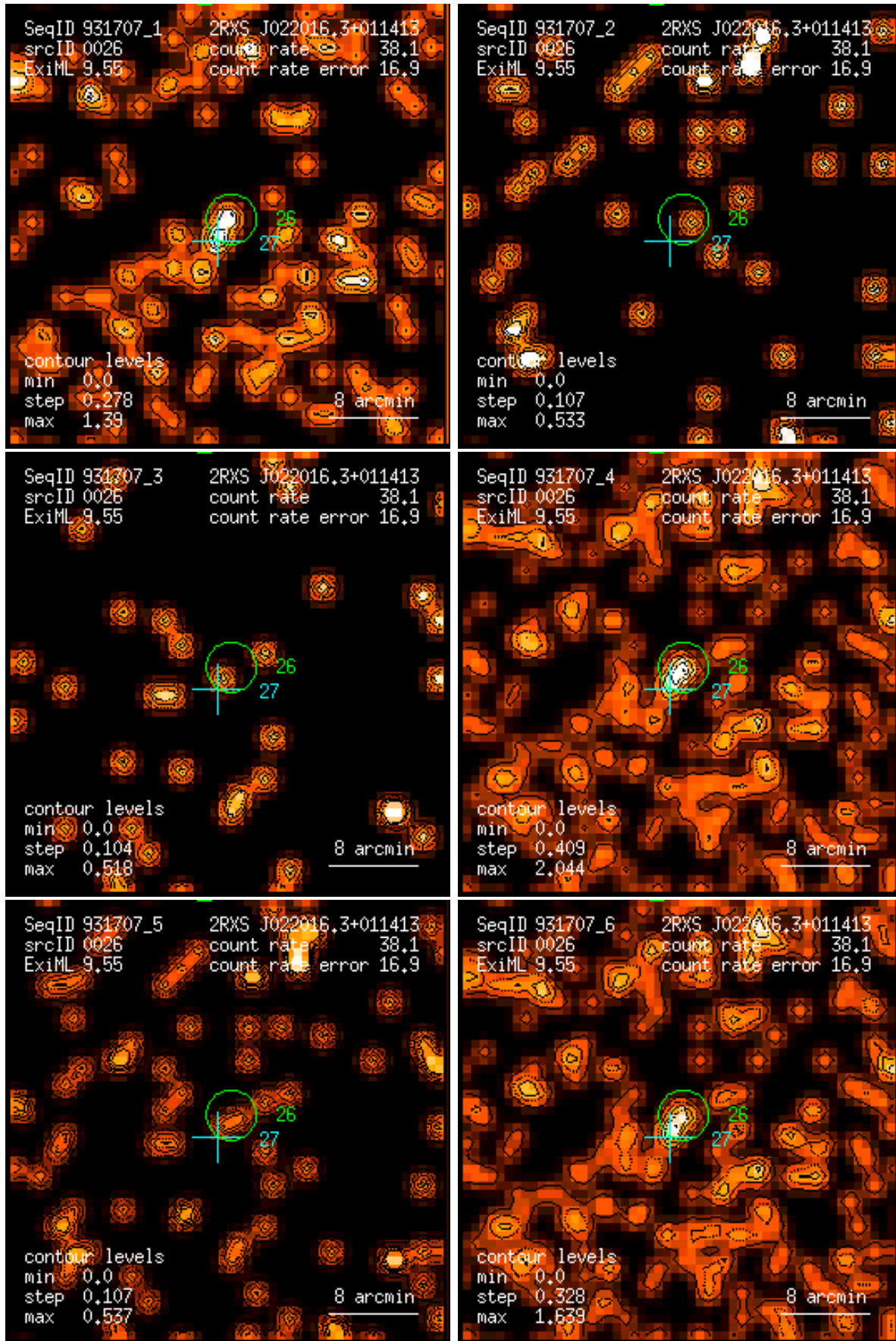
Figure 26: RASS 931707: detection 0026: band rate images, Gaussian filter: (1) PSPC channels 11 – 41, (2) 52 – 90, (3) 91 – 201, (4) 11 – 235, (5) 52 – 201, (6) 11 – 201. Broad band rates in counts/ks. Band rate contour levels in counts/ks/arcmin 2 .
