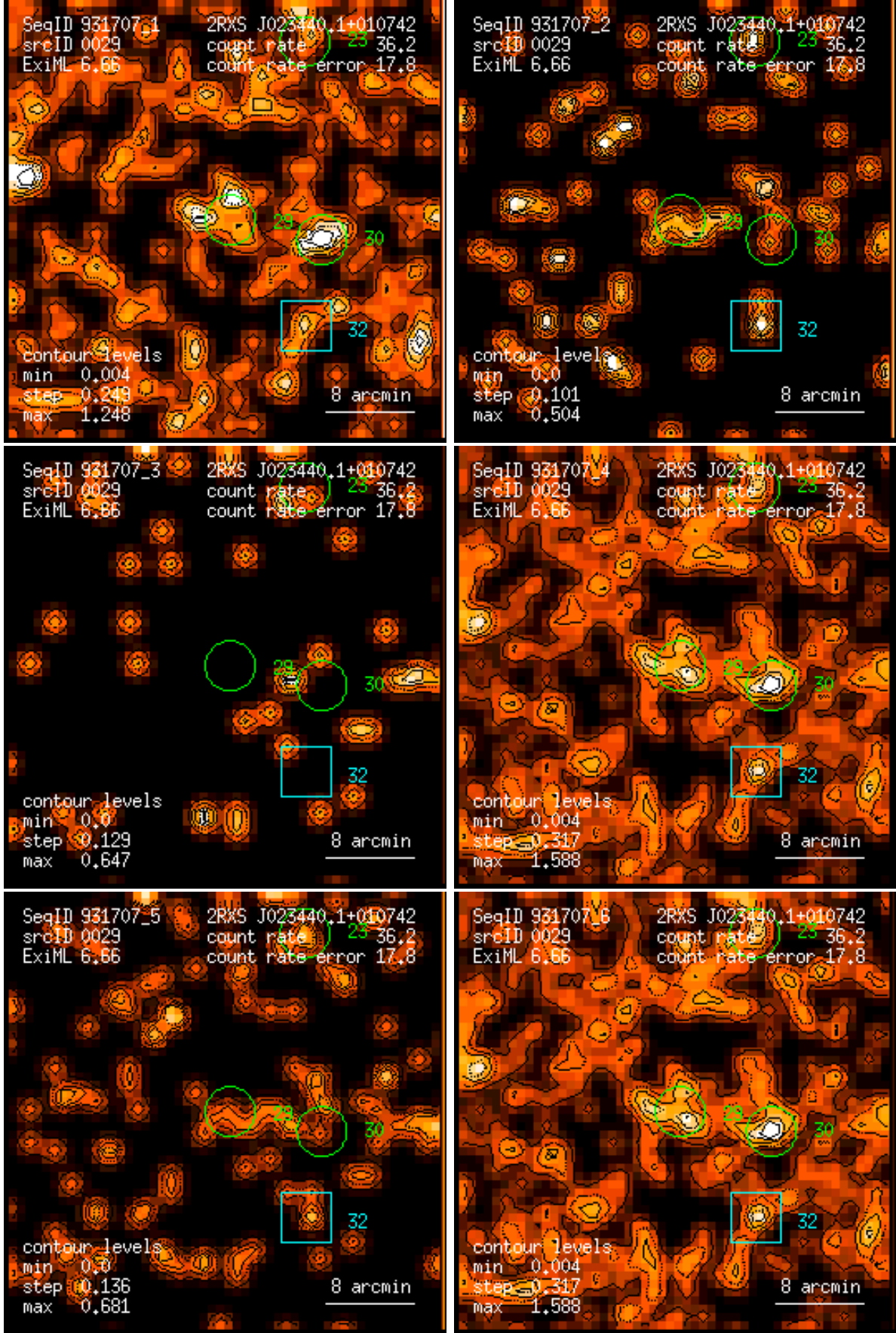
Figure 29: RASS 931707: detection 0029: band rate images, Gaussian filter: (1) PSPC channels 11 – 41, (2) 52 – 90, (3) 91 – 201, (4) 11 – 235, (5) 52 – 201, (6) 11 – 201. Broad band rates in counts/ks. Band rate contour levels in counts/ks/arcmin 2 .
