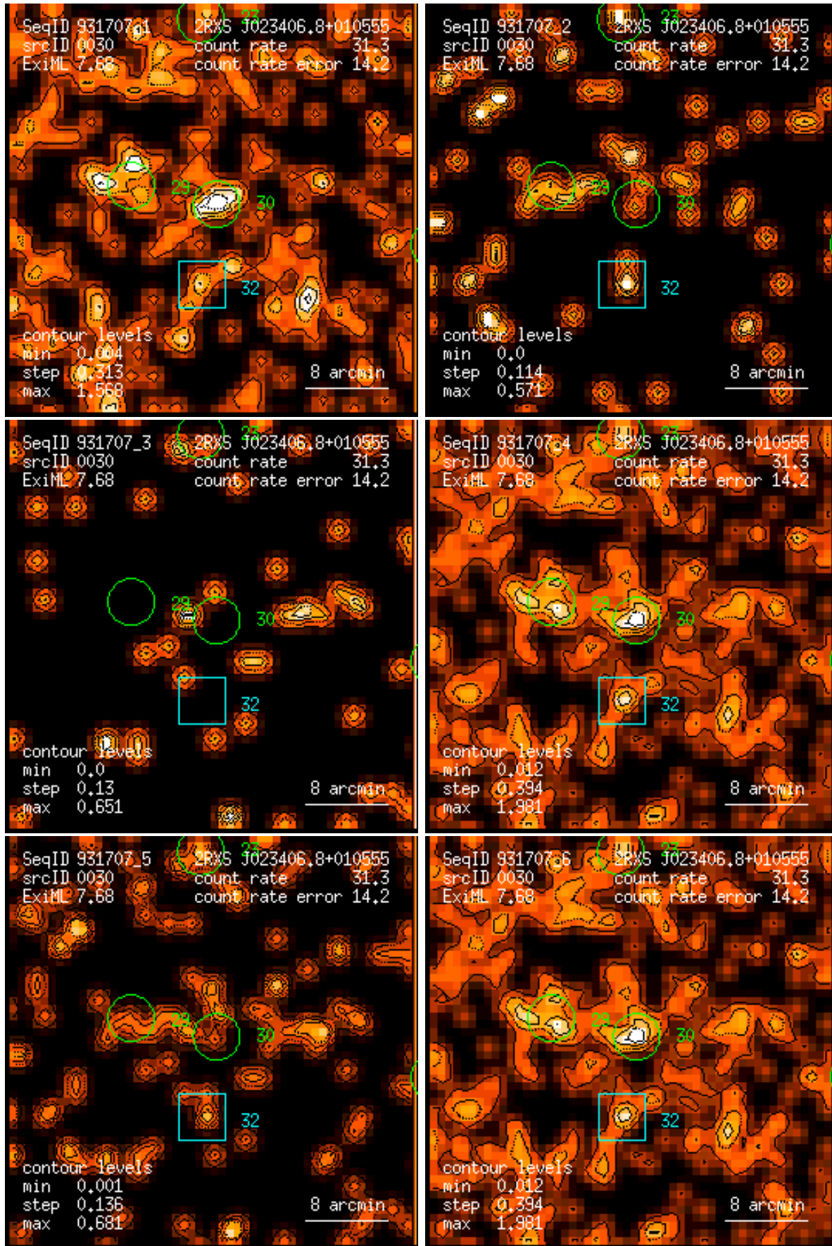
Figure 30: RASS 931707: detection 0030: band rate images, Gaussian filter: (1) PSPC channels 11 – 41, (2) 52 – 90, (3) 91 – 201, (4) 11 – 235, (5) 52 – 201, (6) 11 – 201. Broad band rates in counts/ks. Band rate contour levels in counts/ks/arcmin 2 .
