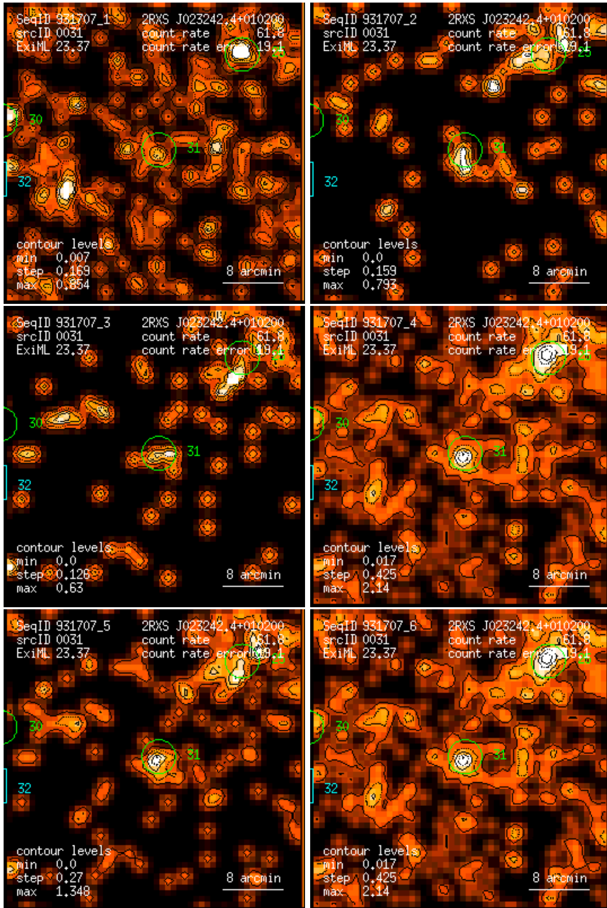
Figure 31: RASS 931707: detection 0031: band rate images, Gaussian filter: (1) PSPC channels 11 – 41, (2) 52 – 90, (3) 91 – 201, (4) 11 – 235, (5) 52 – 201, (6) 11 – 201. Broad band rates in counts/ks. Band rate contour levels in counts/ks/arcmin 2 .
