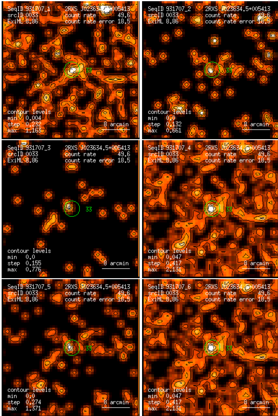
Figure 33: RASS 931707: detection 0033: band rate images, Gaussian filter: (1) PSPC channels 11 – 41, (2) 52 – 90, (3) 91 – 201, (4) 11 – 235, (5) 52 – 201, (6) 11 – 201. Broad band rates in counts/ks. Band rate contour levels in counts/ks/arcmin 2 .
