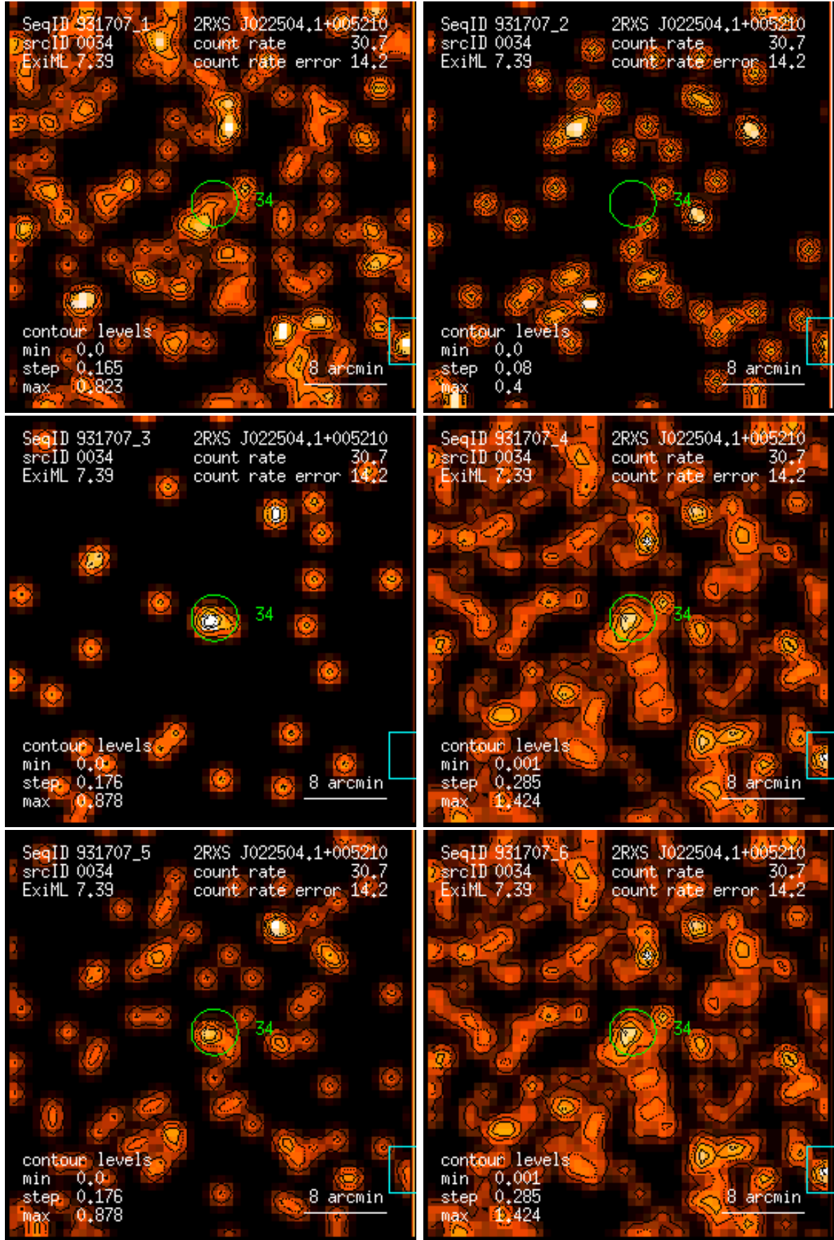
Figure 34: RASS 931707: detection 0034: band rate images, Gaussian filter: (1) PSPC channels 11 – 41, (2) 52 – 90, (3) 91 – 201, (4) 11 – 235, (5) 52 – 201, (6) 11 – 201. Broad band rates in counts/ks. Band rate contour levels in counts/ks/arcmin 2 .
