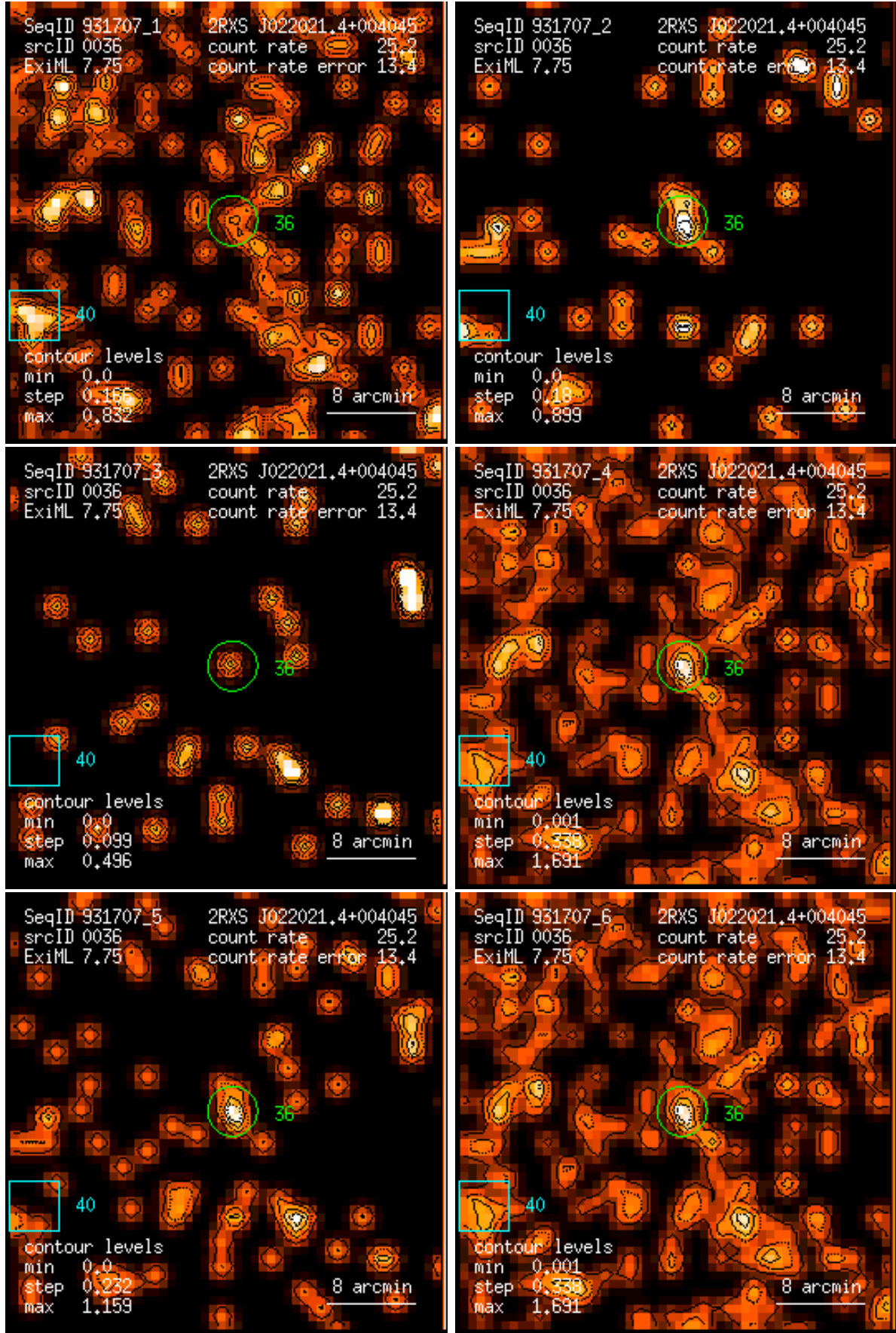
Figure 36: RASS 931707: detection 0036: band rate images, Gaussian filter: (1) PSPC channels 11 – 41, (2) 52 – 90, (3) 91 – 201, (4) 11 – 235, (5) 52 – 201, (6) 11 – 201. Broad band rates in counts/ks. Band rate contour levels in counts/ks/arcmin 2 .
