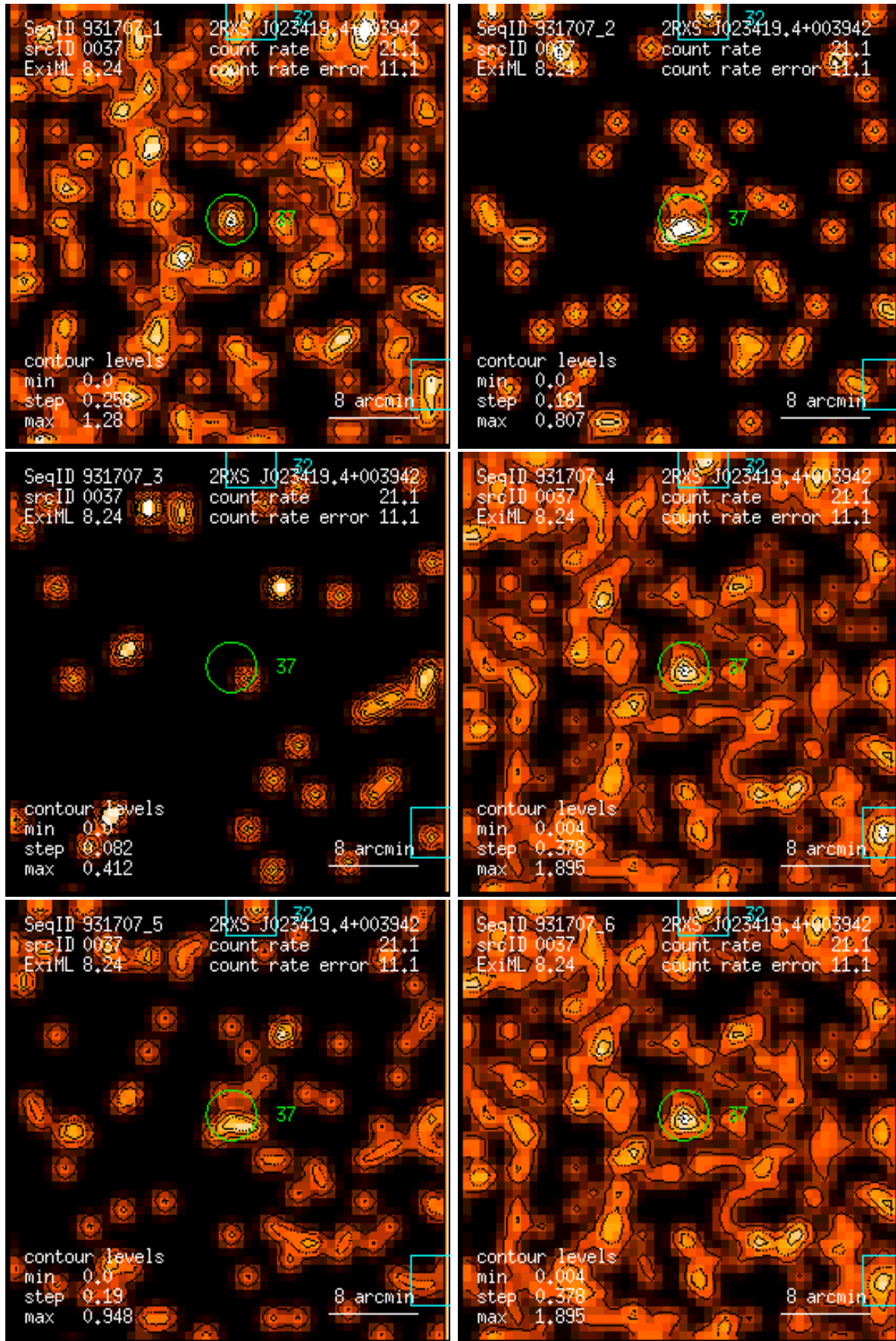
Figure 37: RASS 931707: detection 0037: band rate images, Gaussian filter: (1) PSPC channels 11 – 41, (2) 52 – 90, (3) 91 – 201, (4) 11 – 235, (5) 52 – 201, (6) 11 – 201. Broad band rates in counts/ks. Band rate contour levels in counts/ks/arcmin 2 .
