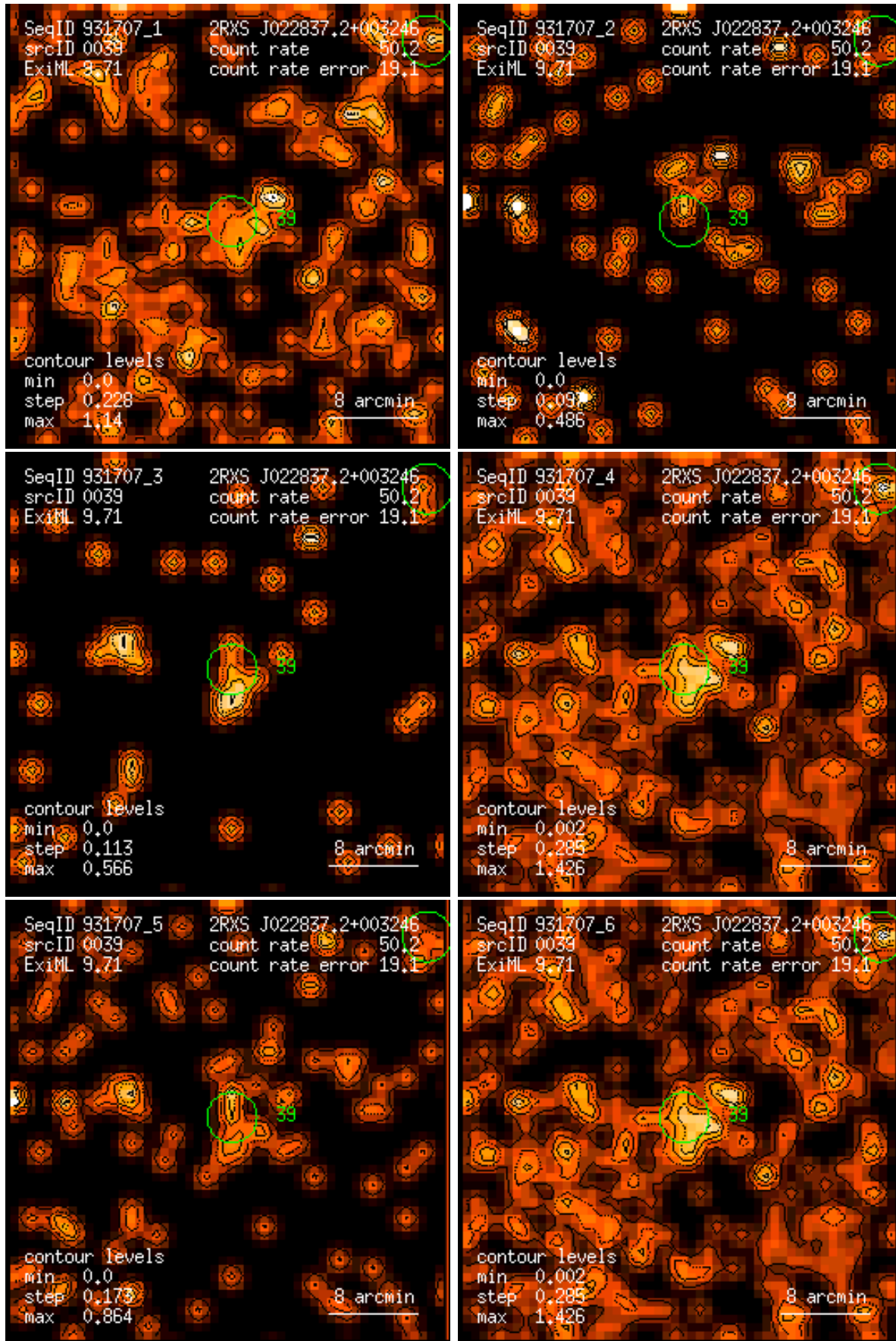
Figure 39: RASS 931707: detection 0039: band rate images, Gaussian filter: (1) PSPC channels 11 – 41, (2) 52 – 90, (3) 91 – 201, (4) 11 – 235, (5) 52 – 201, (6) 11 – 201. Broad band rates in counts/ks. Band rate contour levels in counts/ks/arcmin 2 .
