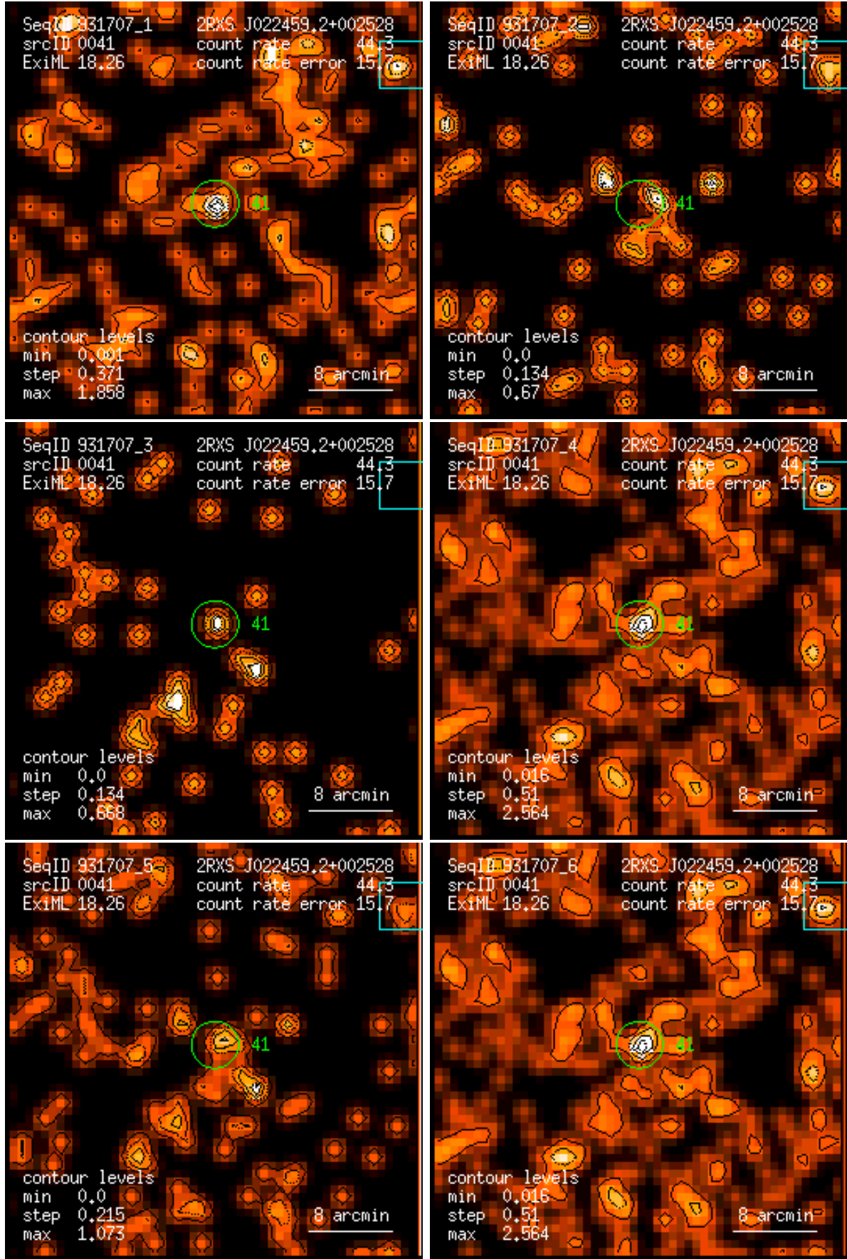
Figure 41: RASS 931707: detection 0041: band rate images, Gaussian filter: (1) PSPC channels 11 – 41, (2) 52 – 90, (3) 91 – 201, (4) 11 – 235, (5) 52 – 201, (6) 11 – 201. Broad band rates in counts/ks. Band rate contour levels in counts/ks/arcmin 2 .
