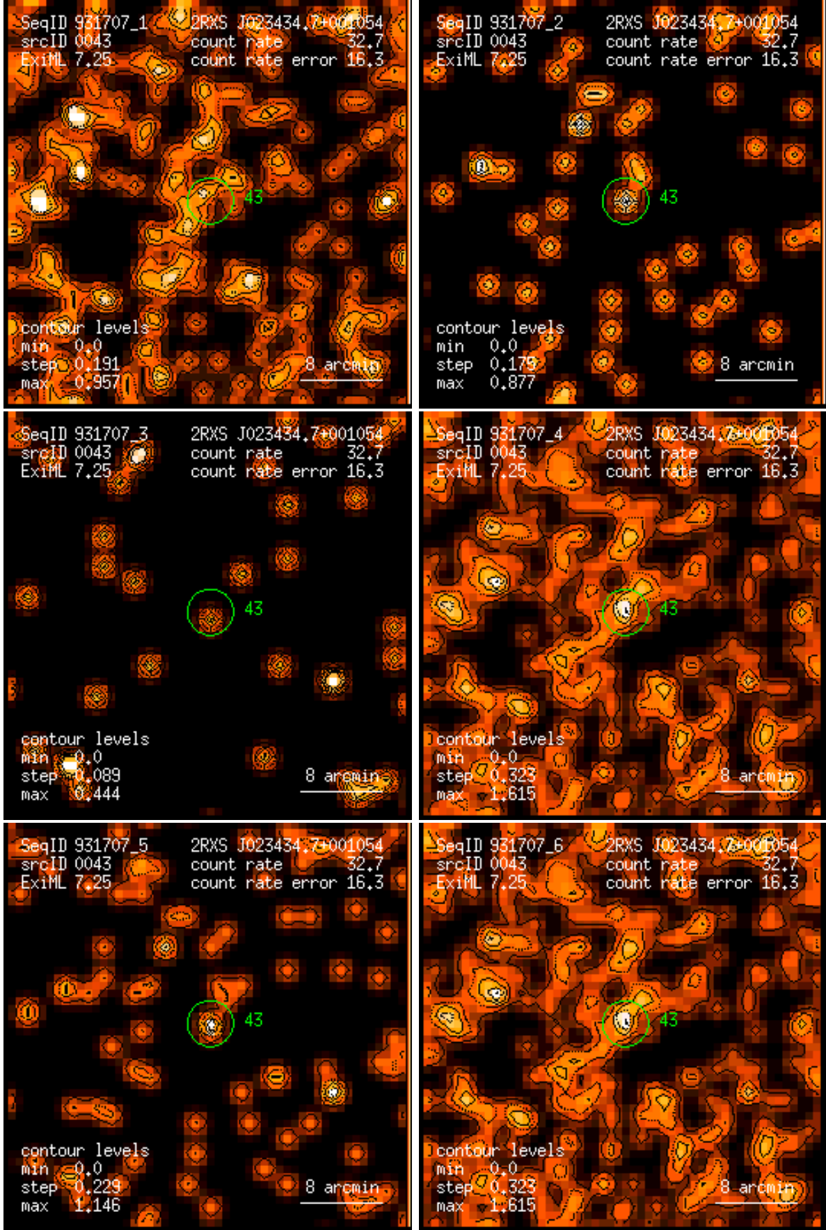
Figure 43: RASS 931707: detection 0043: band rate images, Gaussian filter: (1) PSPC channels 11 – 41, (2) 52 – 90, (3) 91 – 201, (4) 11 – 235, (5) 52 – 201, (6) 11 – 201. Broad band rates in counts/ks. Band rate contour levels in counts/ks/arcmin 2 .
