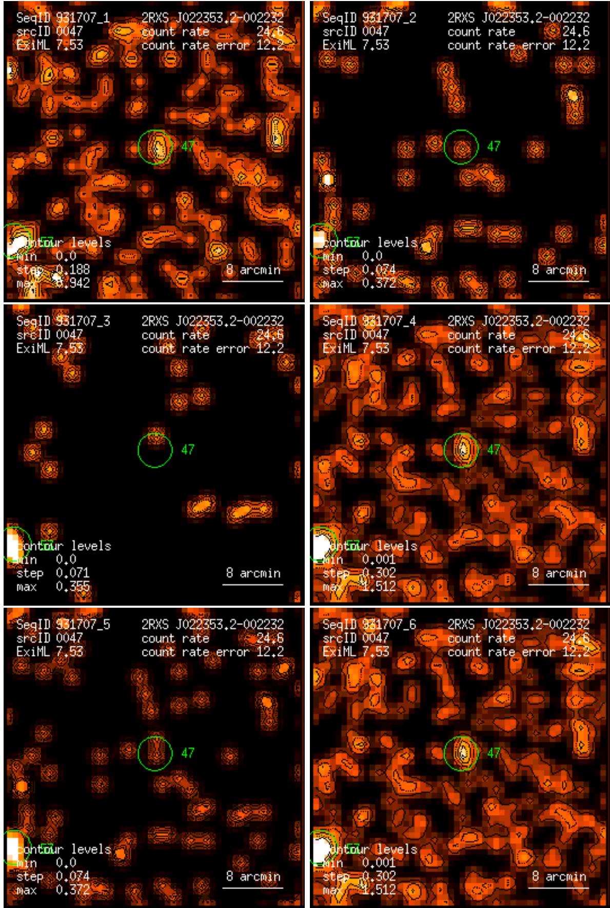
Figure 47: RASS 931707: detection 0047: band rate images, Gaussian filter: (1) PSPC channels 11 – 41, (2) 52 – 90, (3) 91 – 201, (4) 11 – 235, (5) 52 – 201, (6) 11 – 201. Broad band rates in counts/ks. Band rate contour levels in counts/ks/arcmin 2 .
