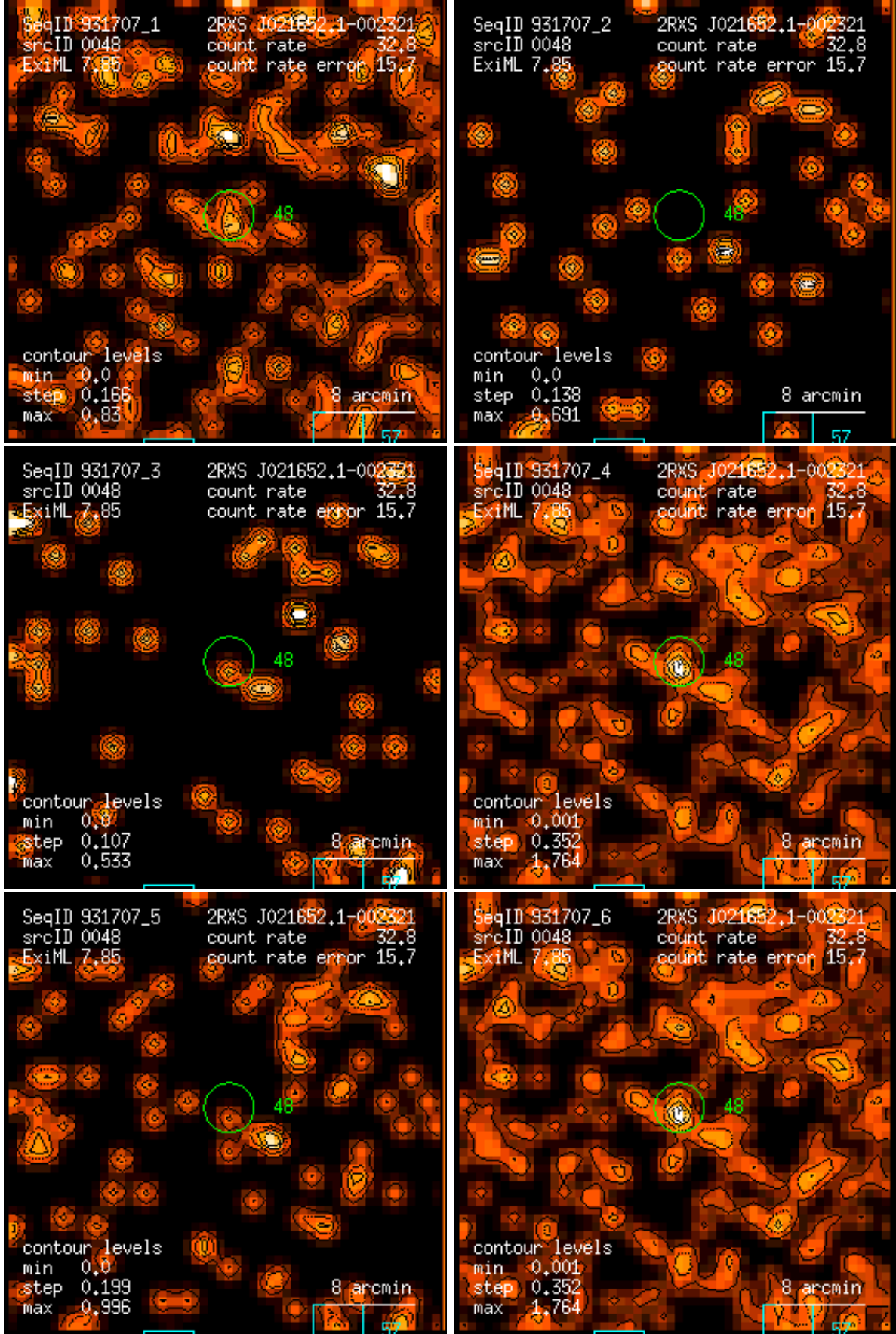
Figure 48: RASS 931707: detection 0048: band rate images, Gaussian filter: (1) PSPC channels 11 – 41, (2) 52 – 90, (3) 91 – 201, (4) 11 – 235, (5) 52 – 201, (6) 11 – 201. Broad band rates in counts/ks. Band rate contour levels in counts/ks/arcmin 2 .
