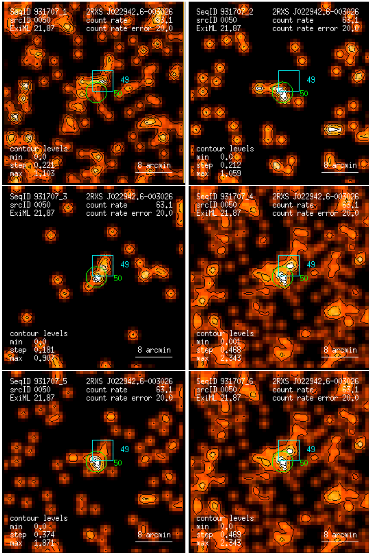
Figure 50: RASS 931707: detection 0050: band rate images, Gaussian filter: (1) PSPC channels 11 – 41, (2) 52 – 90, (3) 91 – 201, (4) 11 – 235, (5) 52 – 201, (6) 11 – 201. Broad band rates in counts/ks. Band rate contour levels in counts/ks/arcmin 2 .
