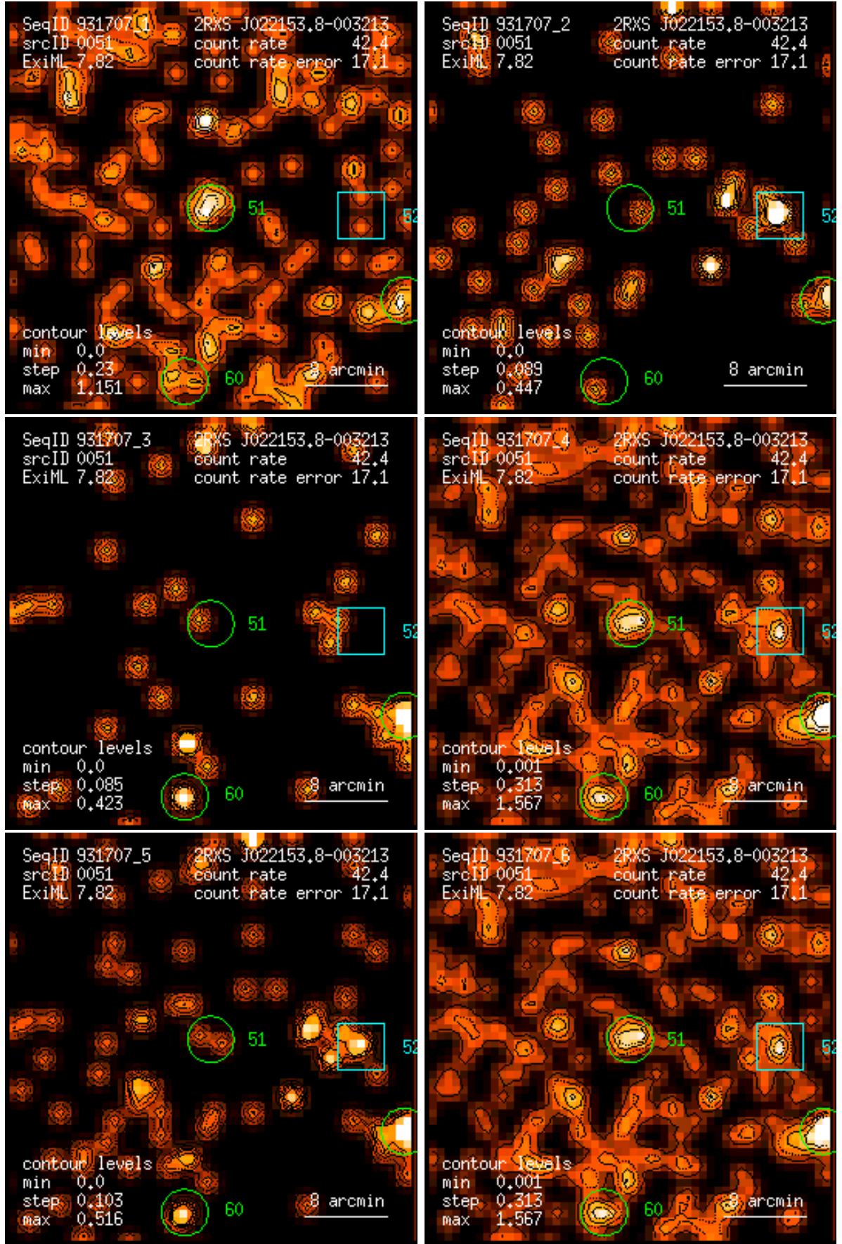
Figure 51: RASS 931707: detection 0051: band rate images, Gaussian filter: (1) PSPC channels 11 – 41, (2) 52 – 90, (3) 91 – 201, (4) 11 – 235, (5) 52 – 201, (6) 11 – 201. Broad band rates in counts/ks. Band rate contour levels in counts/ks/arcmin 2 .
