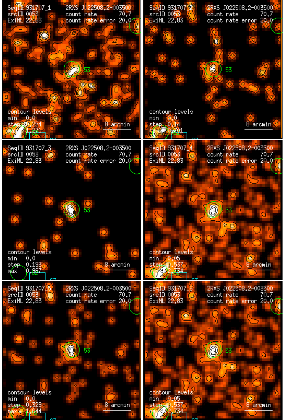
Figure 53: RASS 931707: detection 0053: band rate images, Gaussian filter: (1) PSPC channels 11 – 41, (2) 52 – 90, (3) 91 – 201, (4) 11 – 235, (5) 52 – 201, (6) 11 – 201. Broad band rates in counts/ks. Band rate contour levels in counts/ks/arcmin 2 .
