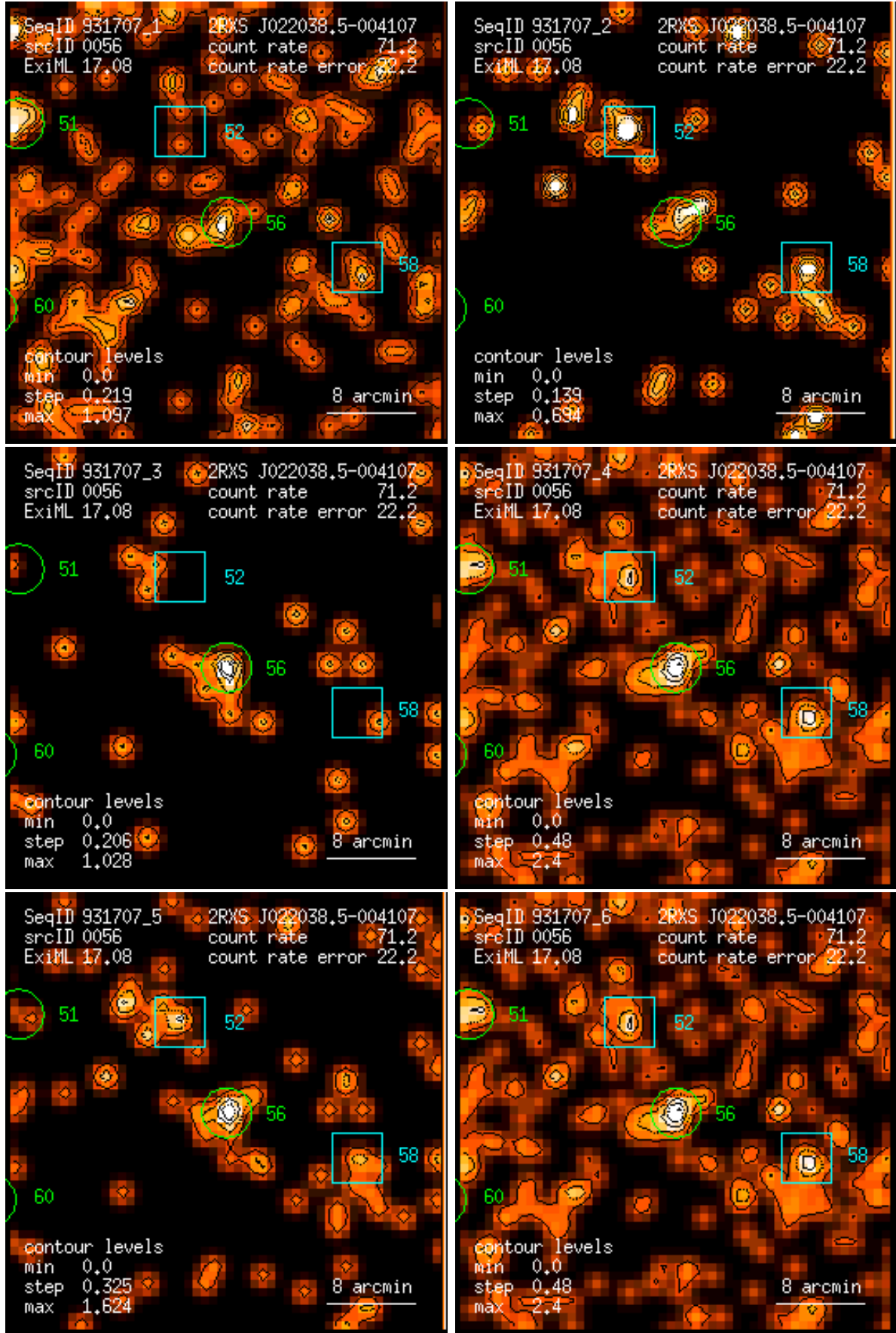
Figure 56: RASS 931707: detection 0056: band rate images, Gaussian filter: (1) PSPC channels 11 – 41, (2) 52 – 90, (3) 91 – 201, (4) 11 – 235, (5) 52 – 201, (6) 11 – 201. Broad band rates in counts/ks. Band rate contour levels in counts/ks/arcmin 2 .
