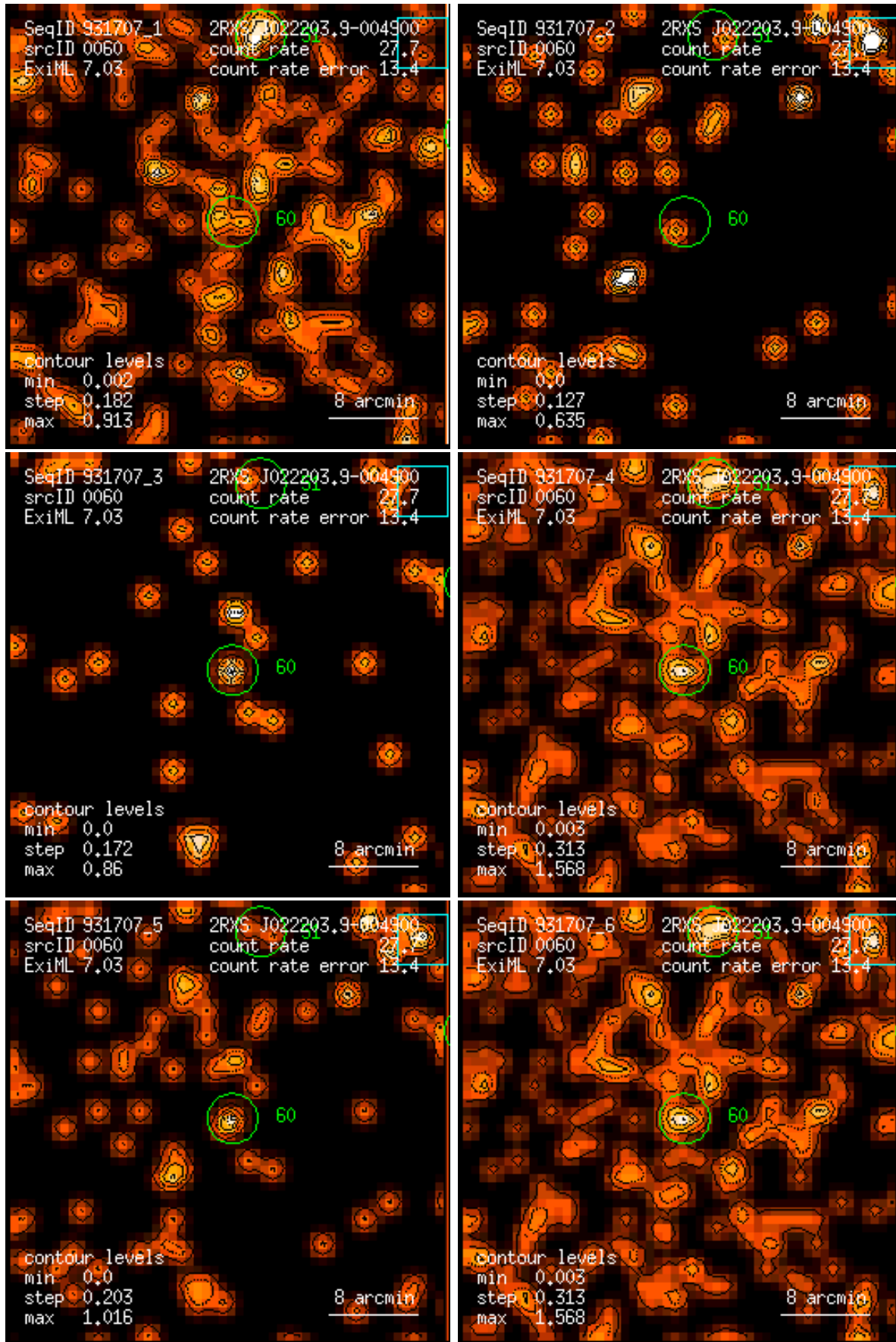
Figure 60: RASS 931707: detection 0060: band rate images, Gaussian filter: (1) PSPC channels 11 – 41, (2) 52 – 90, (3) 91 – 201, (4) 11 – 235, (5) 52 – 201, (6) 11 – 201. Broad band rates in counts/ks. Band rate contour levels in counts/ks/arcmin 2 .
