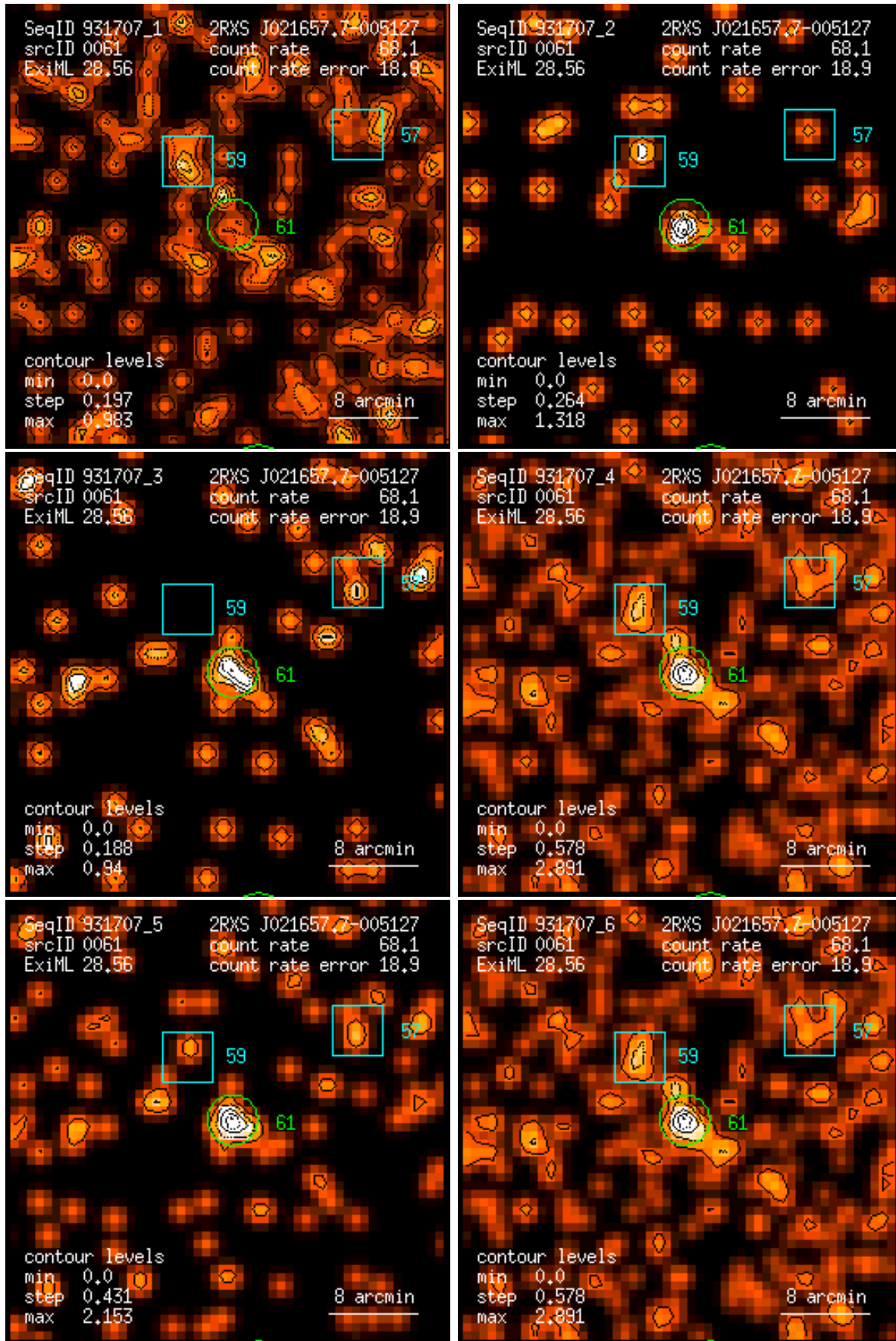
Figure 61: RASS 931707: detection 0061: band rate images, Gaussian filter: (1) PSPC channels 11 – 41, (2) 52 – 90, (3) 91 – 201, (4) 11 – 235, (5) 52 – 201, (6) 11 – 201. Broad band rates in counts/ks. Band rate contour levels in counts/ks/arcmin 2 .
