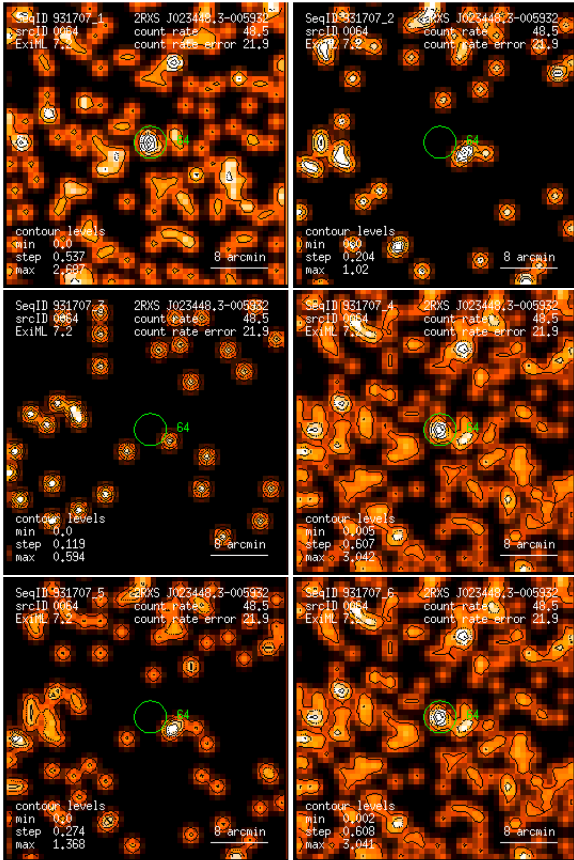
Figure 64: RASS 931707: detection 0064: band rate images, Gaussian filter: (1) PSPC channels 11 – 41, (2) 52 – 90, (3) 91 – 201, (4) 11 – 235, (5) 52 – 201, (6) 11 – 201. Broad band rates in counts/ks. Band rate contour levels in counts/ks/arcmin 2 .
