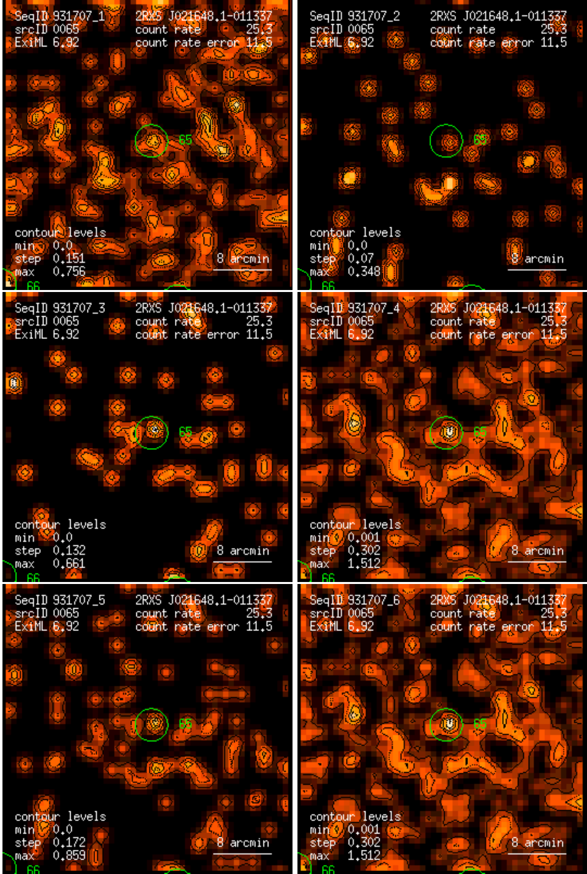
Figure 65: RASS 931707: detection 0065: band rate images, Gaussian filter: (1) PSPC channels 11 – 41, (2) 52 – 90, (3) 91 – 201, (4) 11 – 235, (5) 52 – 201, (6) 11 – 201. Broad band rates in counts/ks. Band rate contour levels in counts/ks/arcmin 2 .
