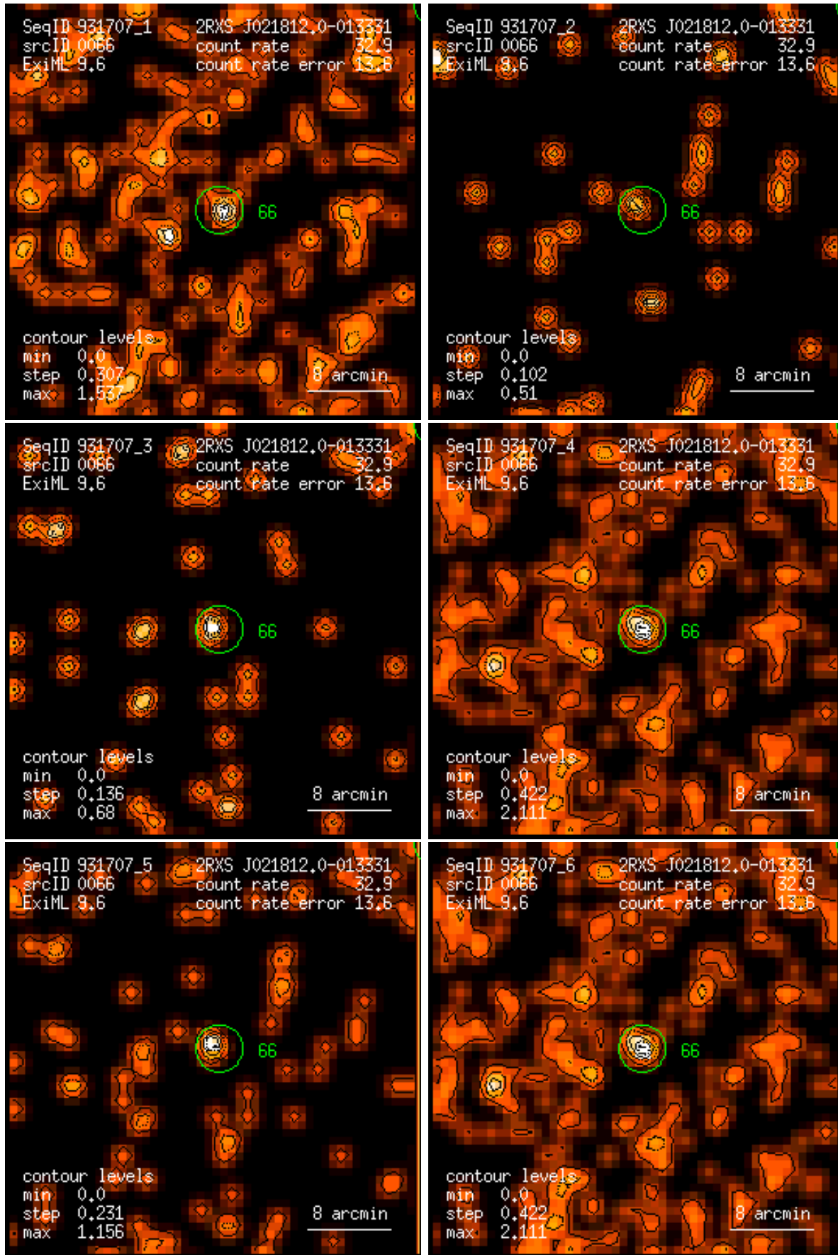
Figure 66: RASS 931707: detection 0066: band rate images, Gaussian filter: (1) PSPC channels 11 – 41, (2) 52 – 90, (3) 91 – 201, (4) 11 – 235, (5) 52 – 201, (6) 11 – 201. Broad band rates in counts/ks. Band rate contour levels in counts/ks/arcmin 2 .
