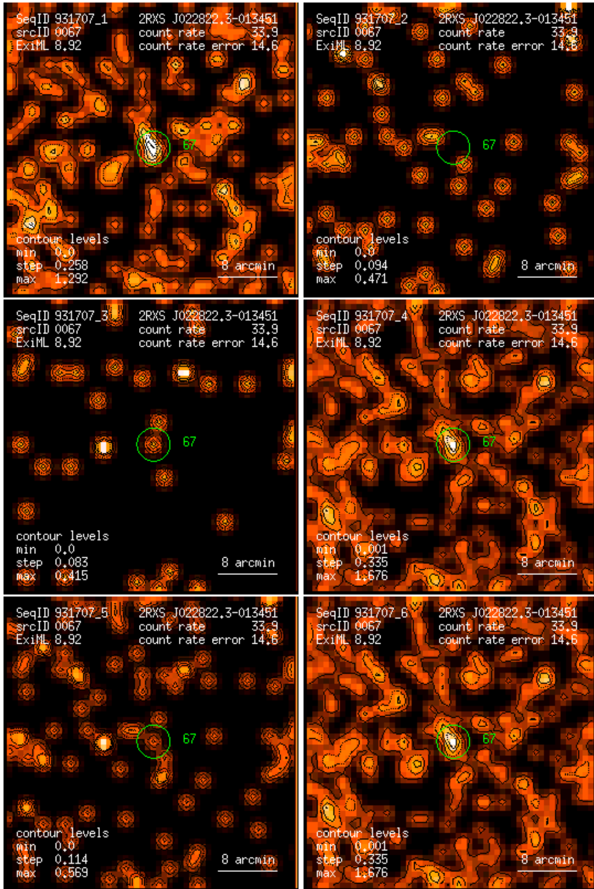
Figure 67: RASS 931707: detection 0067: band rate images, Gaussian filter: (1) PSPC channels 11 – 41, (2) 52 – 90, (3) 91 – 201, (4) 11 – 235, (5) 52 – 201, (6) 11 – 201. Broad band rates in counts/ks. Band rate contour levels in counts/ks/arcmin 2 .
