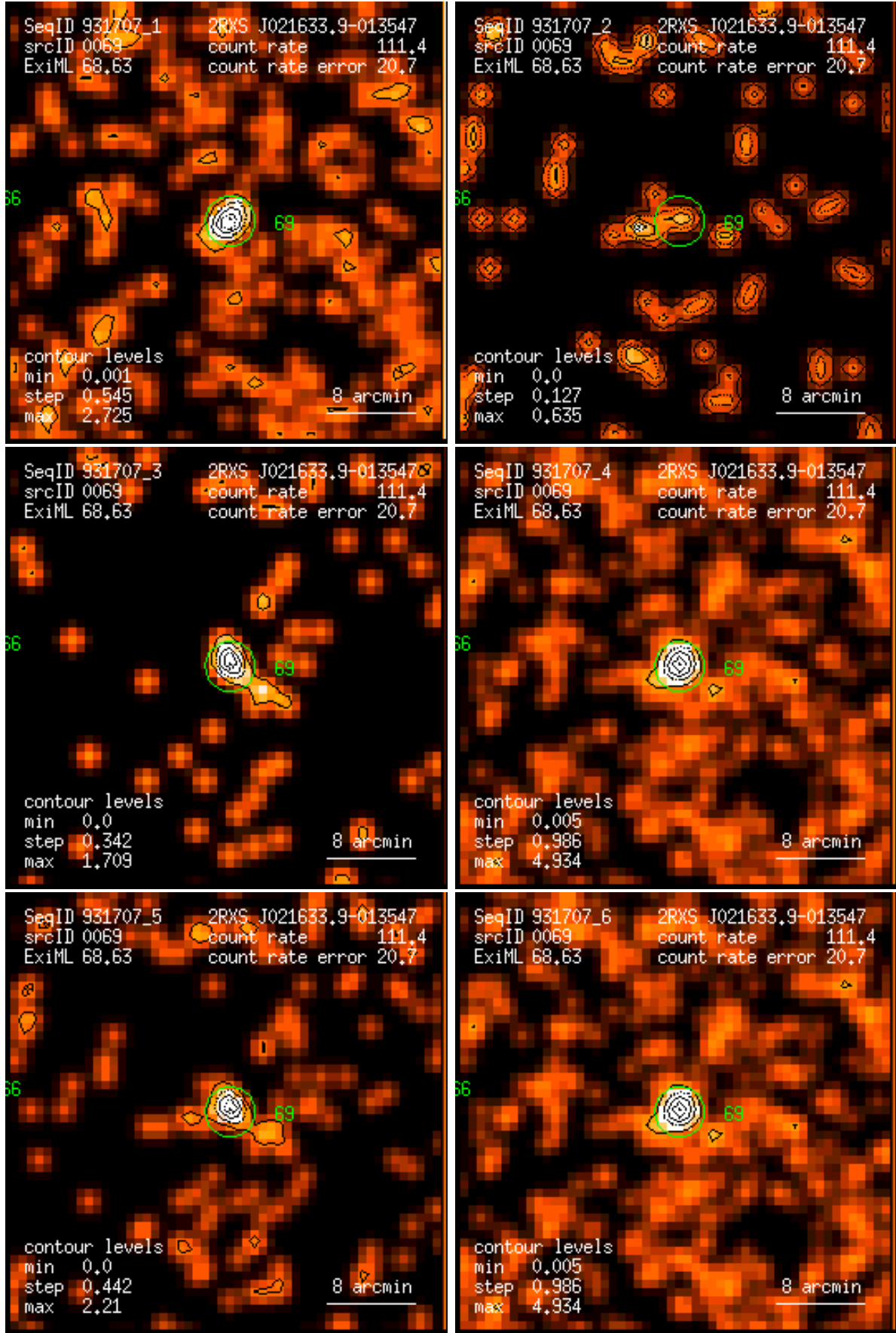
Figure 69: RASS 931707: detection 0069: band rate images, Gaussian filter: (1) PSPC channels 11 – 41, (2) 52 – 90, (3) 91 – 201, (4) 11 – 235, (5) 52 – 201, (6) 11 – 201. Broad band rates in counts/ks. Band rate contour levels in counts/ks/arcmin 2 .
