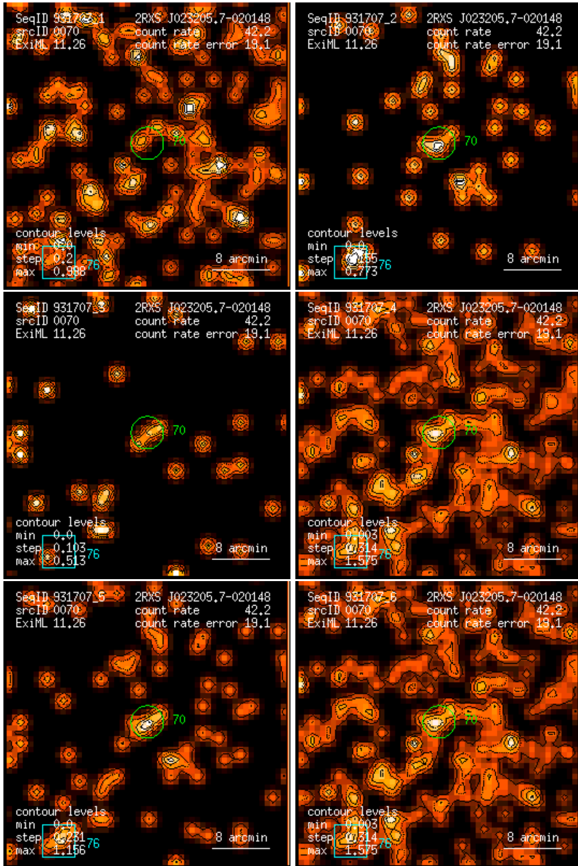
Figure 70: RASS 931707: detection 0070: band rate images, Gaussian filter: (1) PSPC channels 11 – 41, (2) 52 – 90, (3) 91 – 201, (4) 11 – 235, (5) 52 – 201, (6) 11 – 201. Broad band rates in counts/ks. Band rate contour levels in counts/ks/arcmin 2 .
