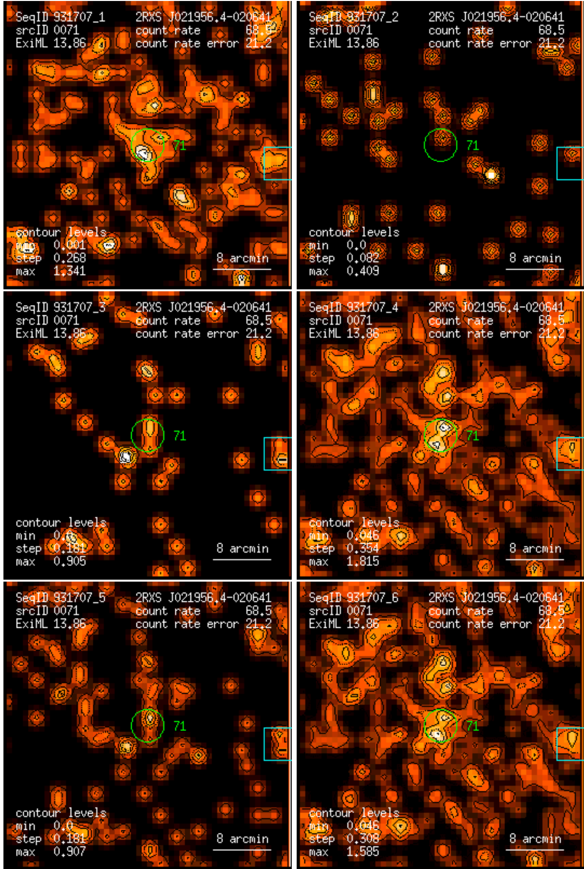
Figure 71: RASS 931707: detection 0071: band rate images, Gaussian filter: (1) PSPC channels 11 – 41, (2) 52 – 90, (3) 91 – 201, (4) 11 – 235, (5) 52 – 201, (6) 11 – 201. Broad band rates in counts/ks. Band rate contour levels in counts/ks/arcmin 2 .
