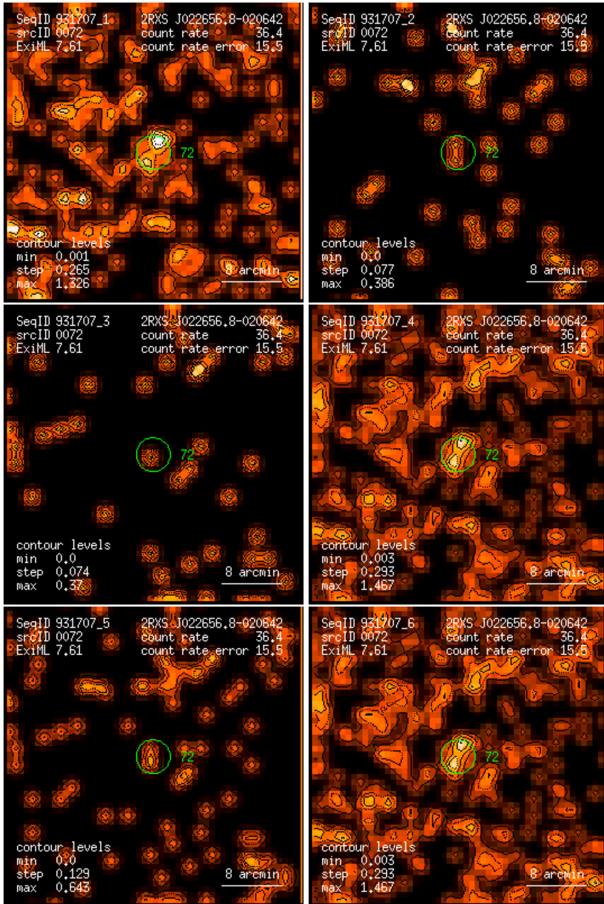
Figure 72: RASS 931707: detection 0072: band rate images, Gaussian filter: (1) PSPC channels 11 – 41, (2) 52 – 90, (3) 91 – 201, (4) 11 – 235, (5) 52 – 201, (6) 11 – 201. Broad band rates in counts/ks. Band rate contour levels in counts/ks/arcmin 2 .
