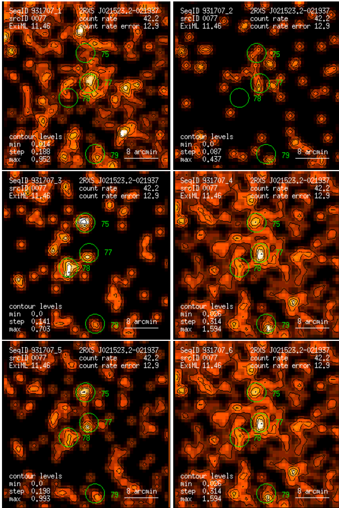
Figure 77: RASS 931707: detection 0077: band rate images, Gaussian filter: (1) PSPC channels 11 – 41, (2) 52 – 90, (3) 91 – 201, (4) 11 – 235, (5) 52 – 201, (6) 11 – 201. Broad band rates in counts/ks. Band rate contour levels in counts/ks/arcmin 2 .
