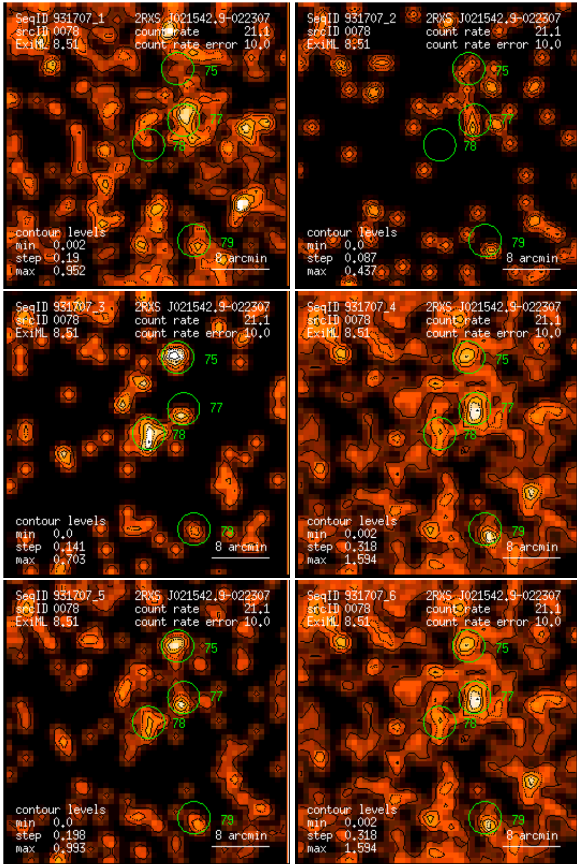
Figure 78: RASS 931707: detection 0078: band rate images, Gaussian filter: (1) PSPC channels 11 – 41, (2) 52 – 90, (3) 91 – 201, (4) 11 – 235, (5) 52 – 201, (6) 11 – 201. Broad band rates in counts/ks. Band rate contour levels in counts/ks/arcmin 2 .
