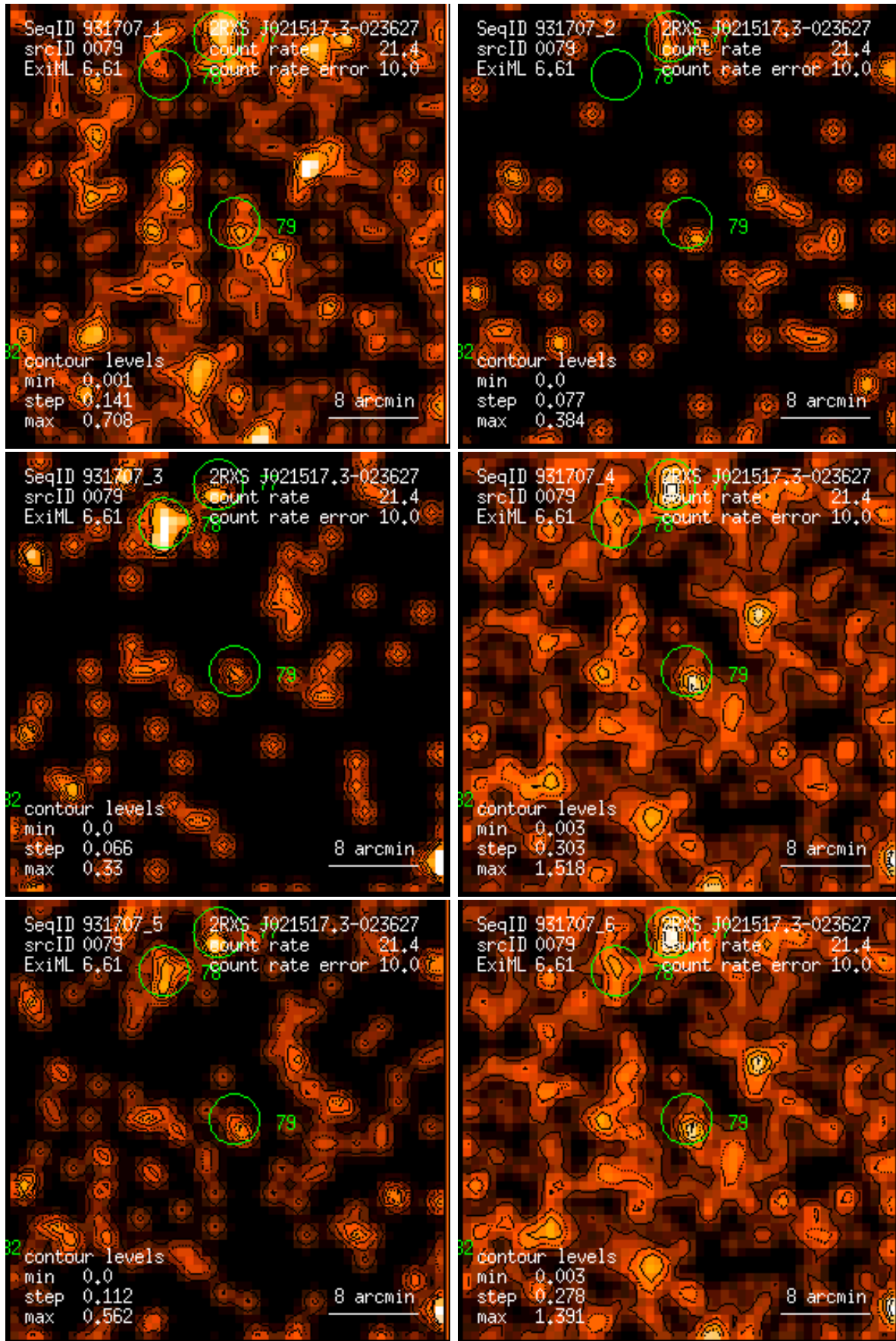
Figure 79: RASS 931707: detection 0079: band rate images, Gaussian filter: (1) PSPC channels 11 – 41, (2) 52 – 90, (3) 91 – 201, (4) 11 – 235, (5) 52 – 201, (6) 11 – 201. Broad band rates in counts/ks. Band rate contour levels in counts/ks/arcmin 2 .
