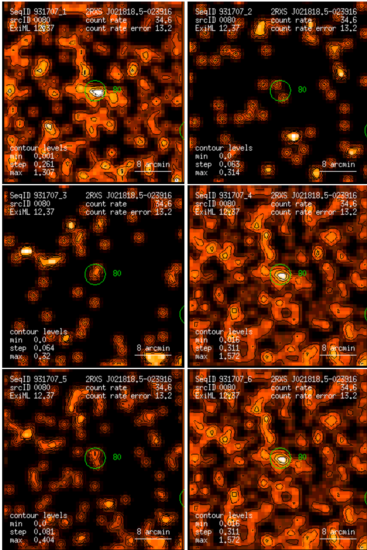
Figure 80: RASS 931707: detection 0080: band rate images, Gaussian filter: (1) PSPC channels 11 – 41, (2) 52 – 90, (3) 91 – 201, (4) 11 – 235, (5) 52 – 201, (6) 11 – 201. Broad band rates in counts/ks. Band rate contour levels in counts/ks/arcmin 2 .
