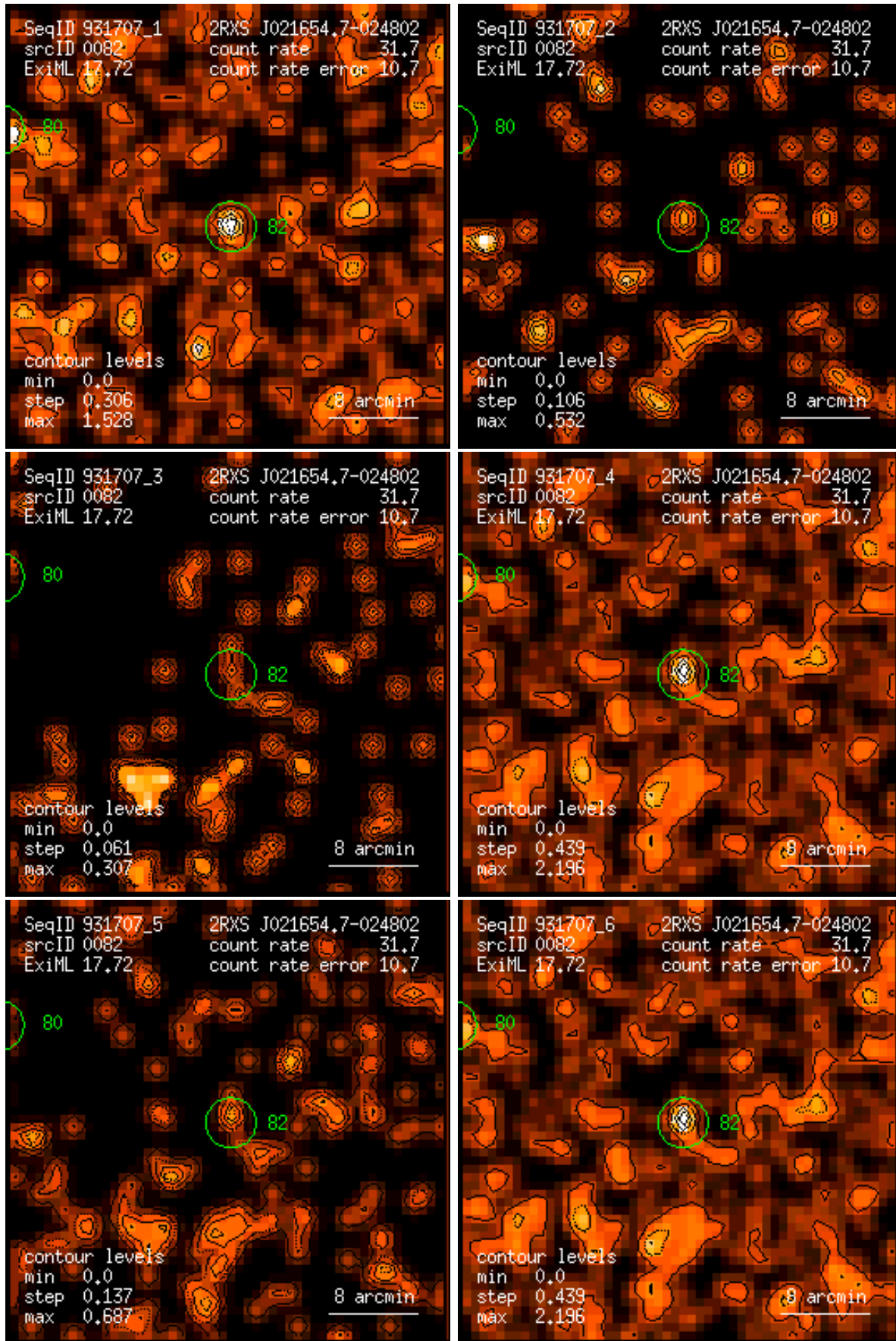
Figure 82: RASS 931707: detection 0082: band rate images, Gaussian filter: (1) PSPC channels 11 – 41, (2) 52 – 90, (3) 91 – 201, (4) 11 – 235, (5) 52 – 201, (6) 11 – 201. Broad band rates in counts/ks. Band rate contour levels in counts/ks/arcmin 2 .
