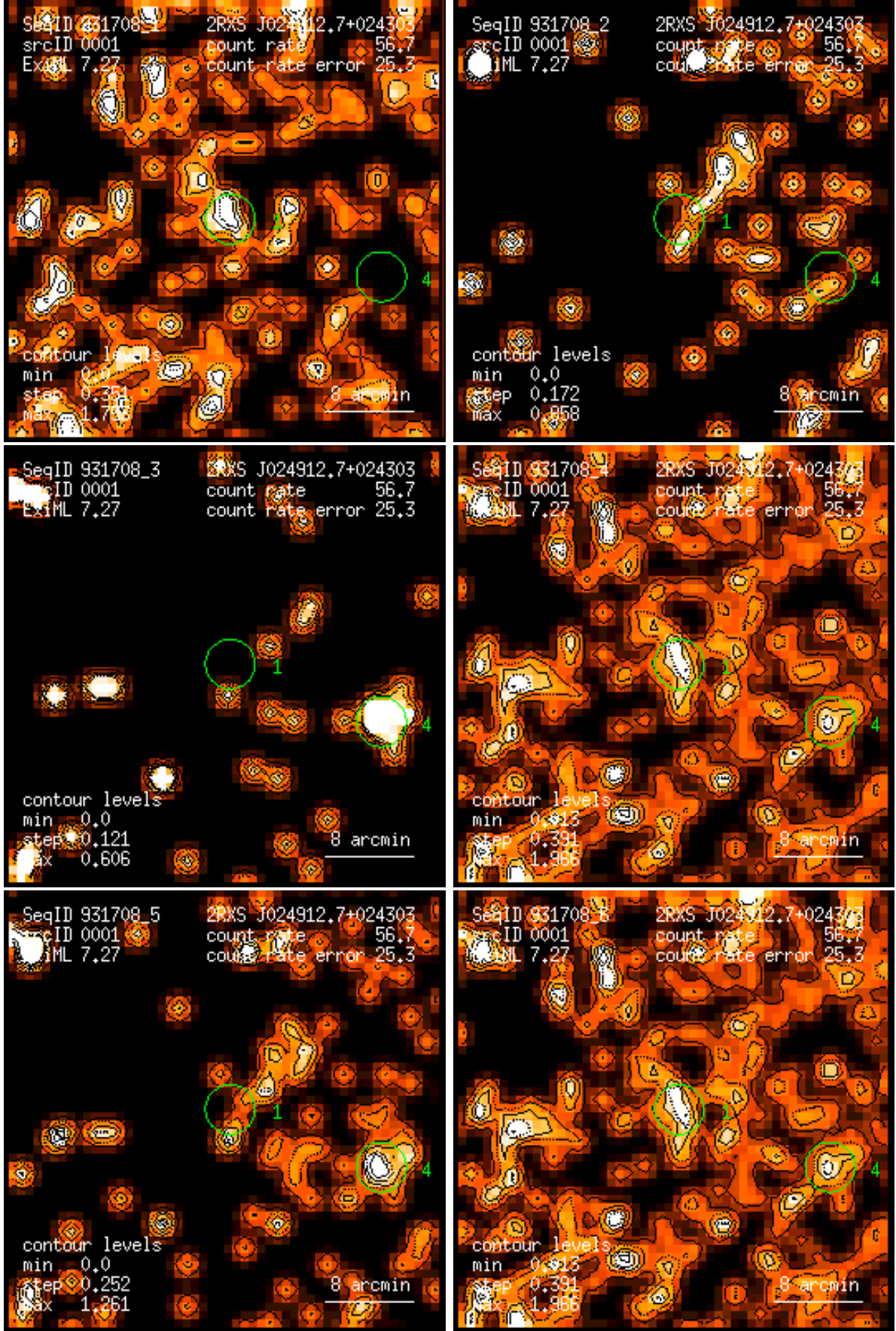
Figure 1: RASS 931708: detection 0001: band rate images, Gaussian filter: (1) PSPC channels 11 – 41, (2) 52 – 90, (3) 91 – 201, (4) 11 – 235, (5) 52 – 201, (6) 11 – 201. Broad band rates in counts/ks. Band rate contour levels in counts/ks/arcmin 2 .
