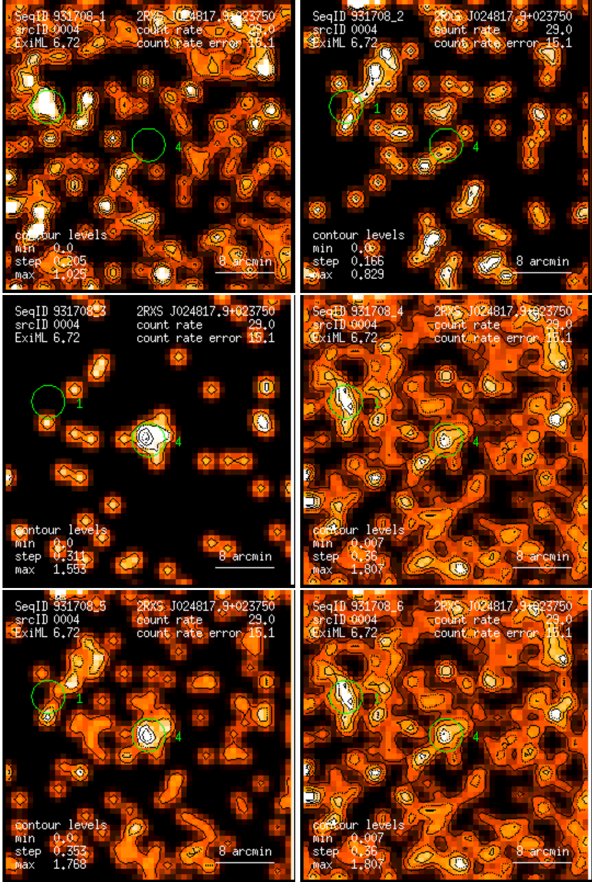
Figure 4: RASS 931708: detection 0004: band rate images, Gaussian filter: (1) PSPC channels 11 – 41, (2) 52 – 90, (3) 91 – 201, (4) 11 – 235, (5) 52 – 201, (6) 11 – 201. Broad band rates in counts/ks. Band rate contour levels in counts/ks/arcmin 2 .
