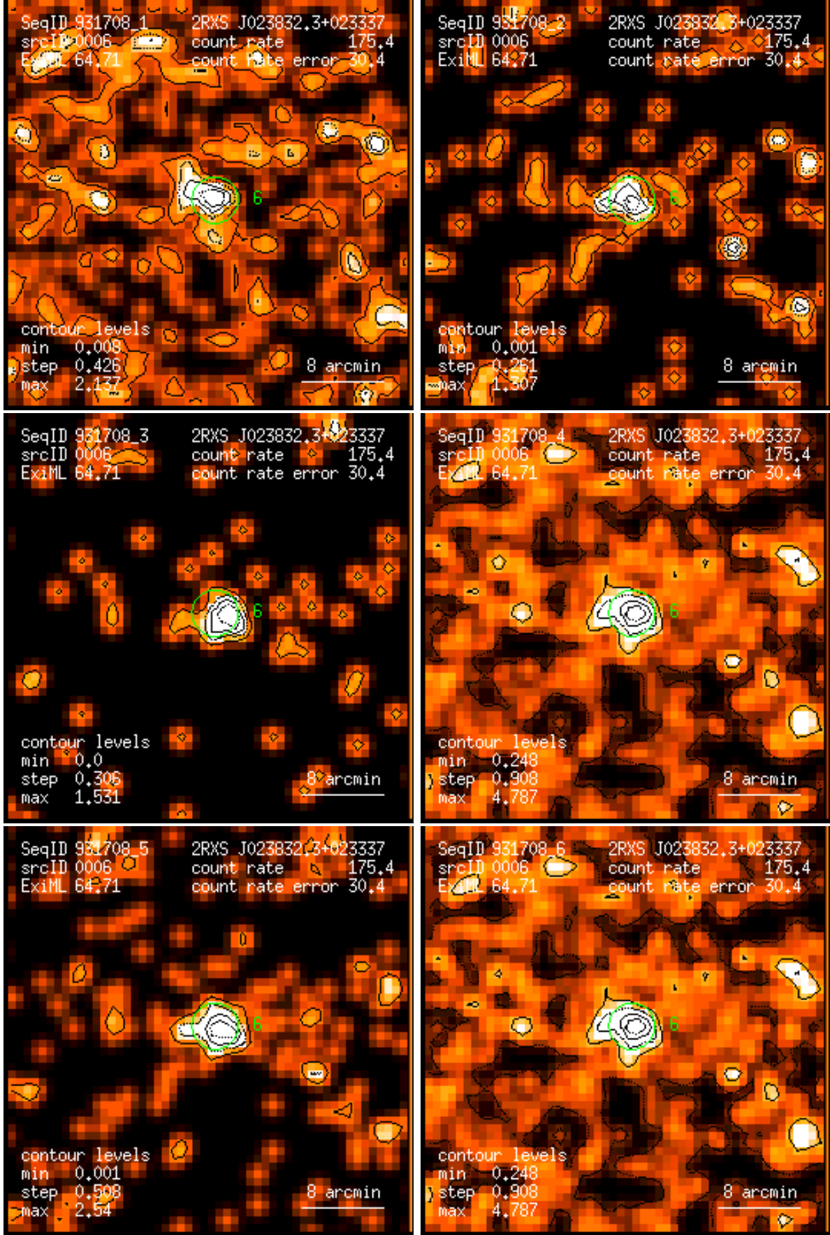
Figure 6: RASS 931708: detection 0006: band rate images, Gaussian filter: (1) PSPC channels 11 – 41, (2) 52 – 90, (3) 91 – 201, (4) 11 – 235, (5) 52 – 201, (6) 11 – 201. Broad band rates in counts/ks. Band rate contour levels in counts/ks/arcmin 2 .
