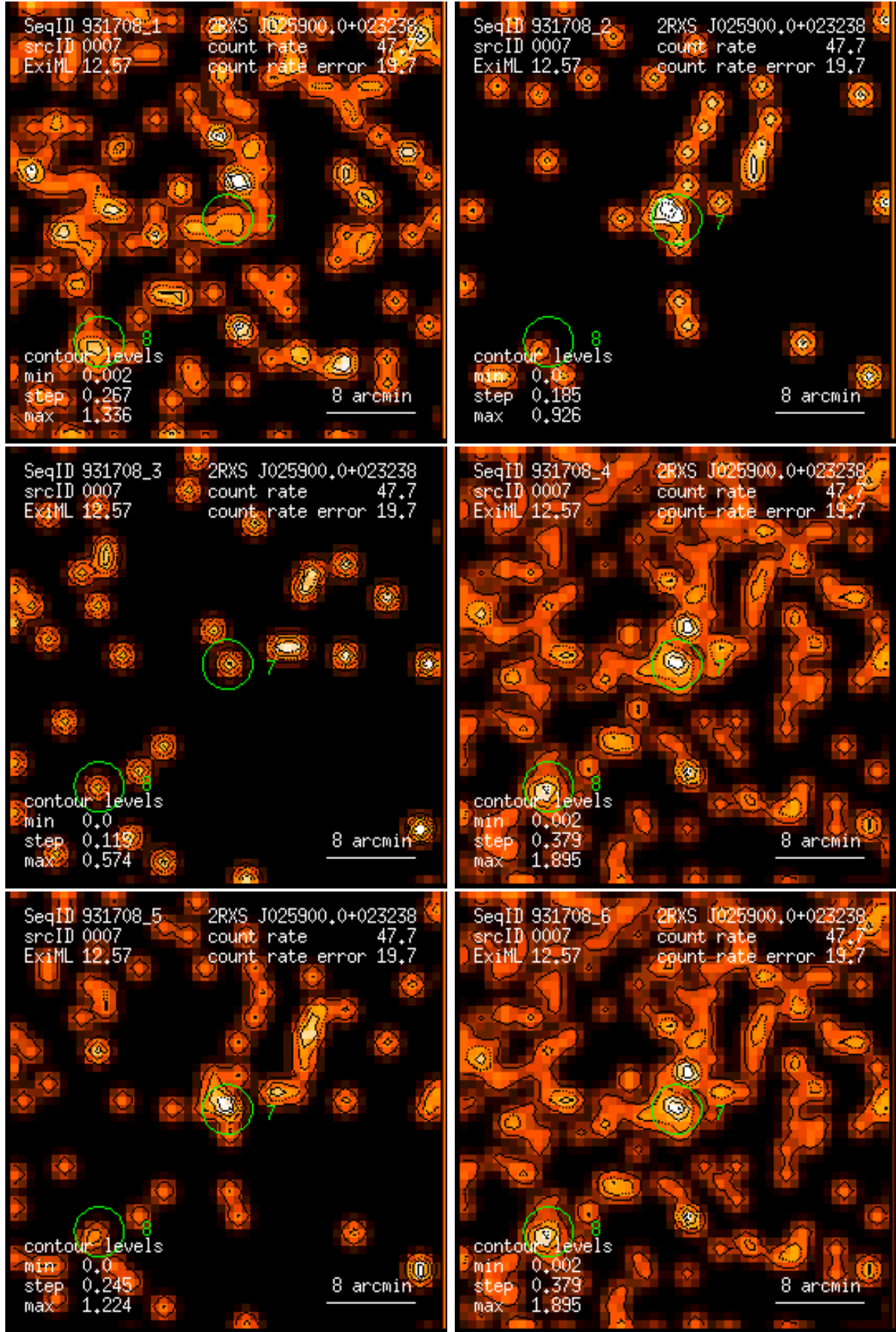
Figure 7: RASS 931708: detection 0007: band rate images, Gaussian filter: (1) PSPC channels 11 – 41, (2) 52 – 90, (3) 91 – 201, (4) 11 – 235, (5) 52 – 201, (6) 11 – 201. Broad band rates in counts/ks. Band rate contour levels in counts/ks/arcmin 2 .
