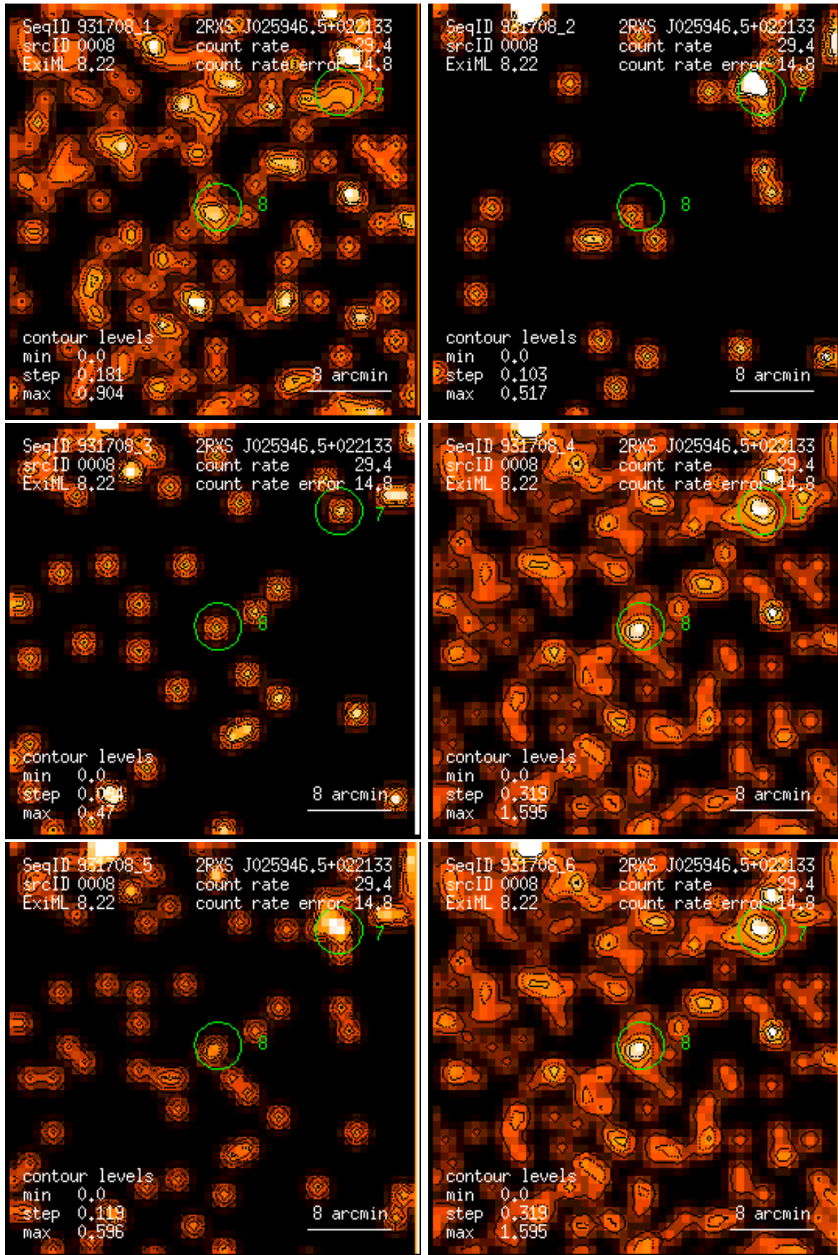
Figure 8: RASS 931708: detection 0008: band rate images, Gaussian filter: (1) PSPC channels 11 – 41, (2) 52 – 90, (3) 91 – 201, (4) 11 – 235, (5) 52 – 201, (6) 11 – 201. Broad band rates in counts/ks. Band rate contour levels in counts/ks/arcmin 2 .
